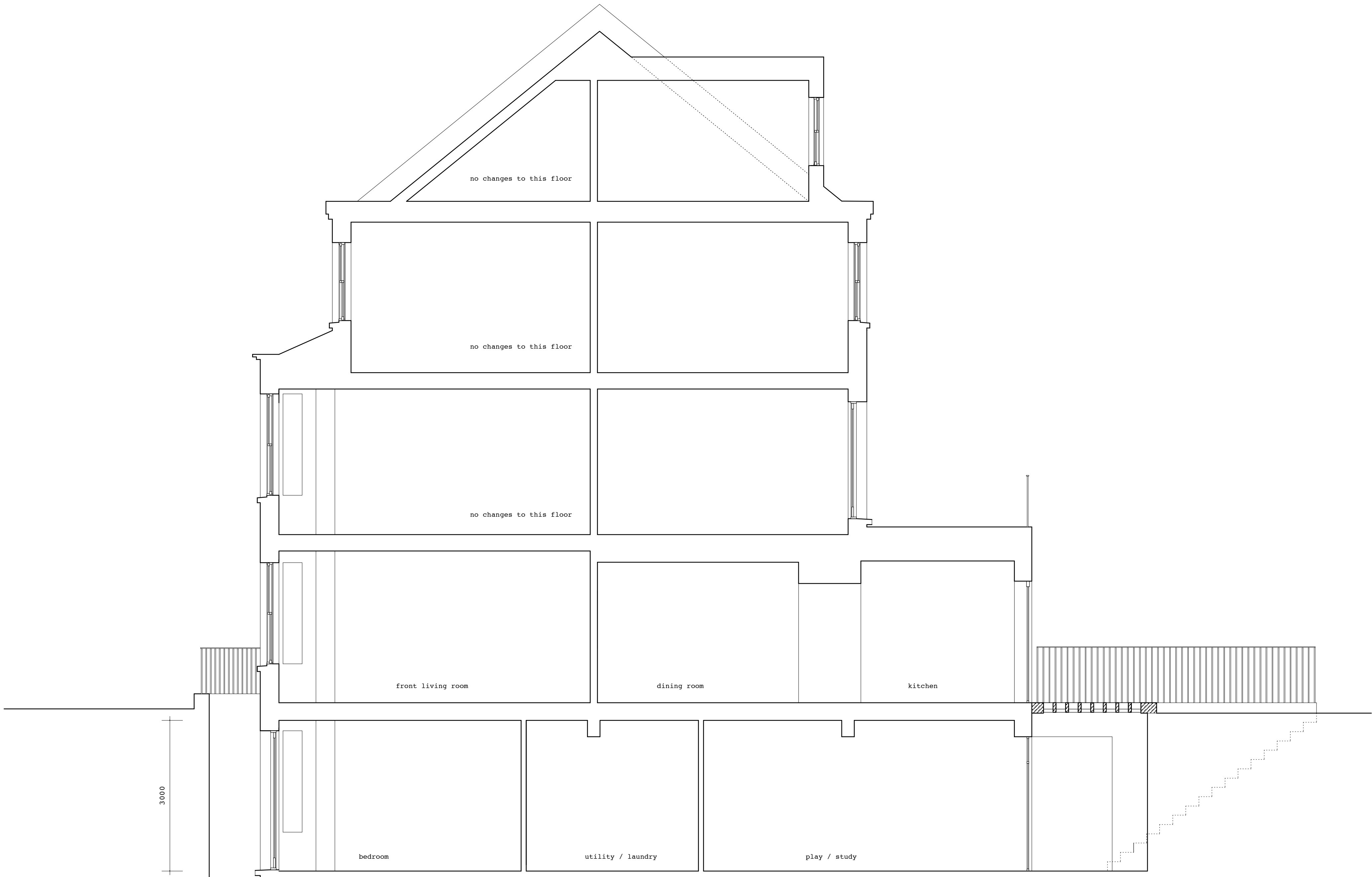
PROPOSED - SECTION B - B
