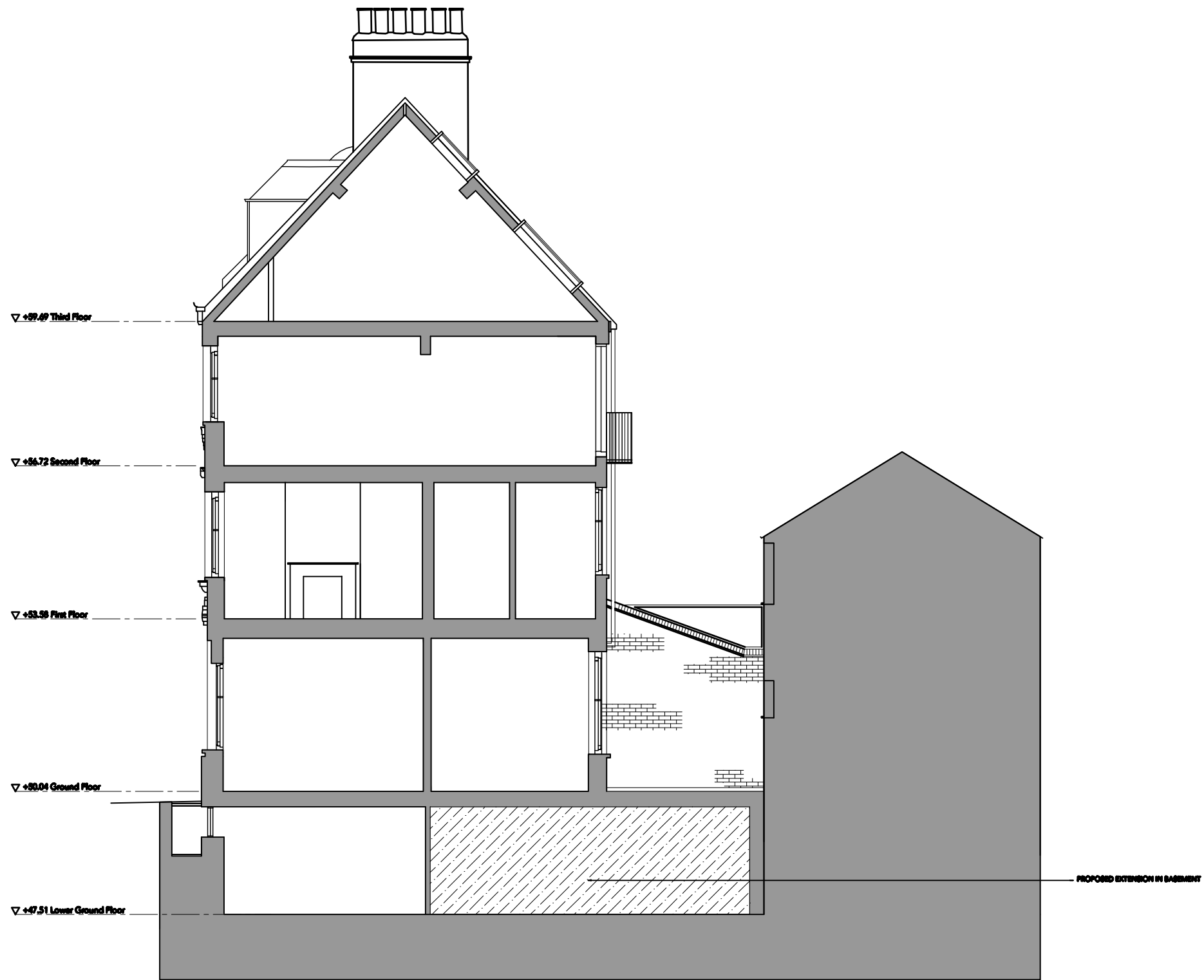
1 Proposed Section A scale 1:80
