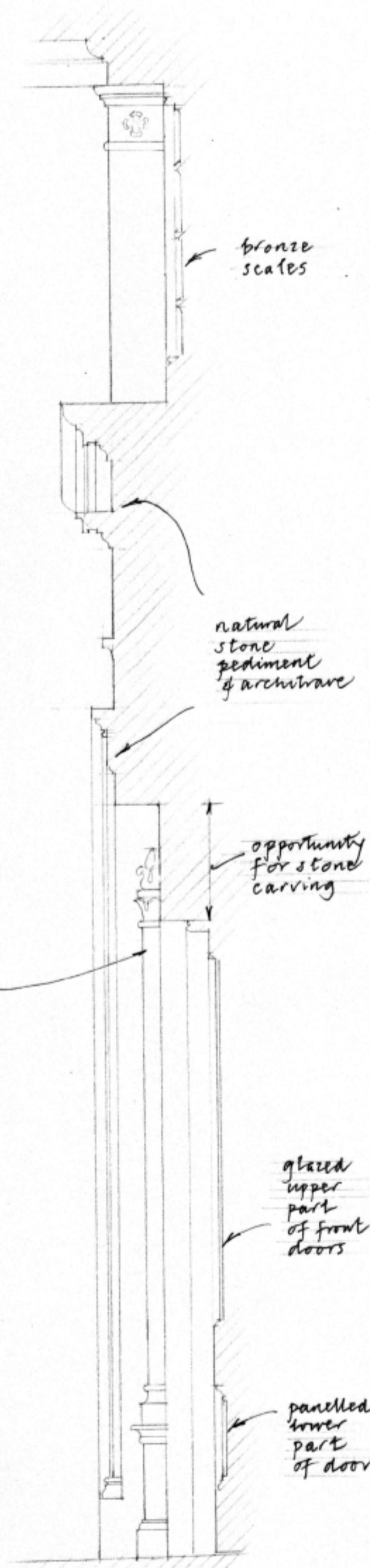
Section thro front doors
