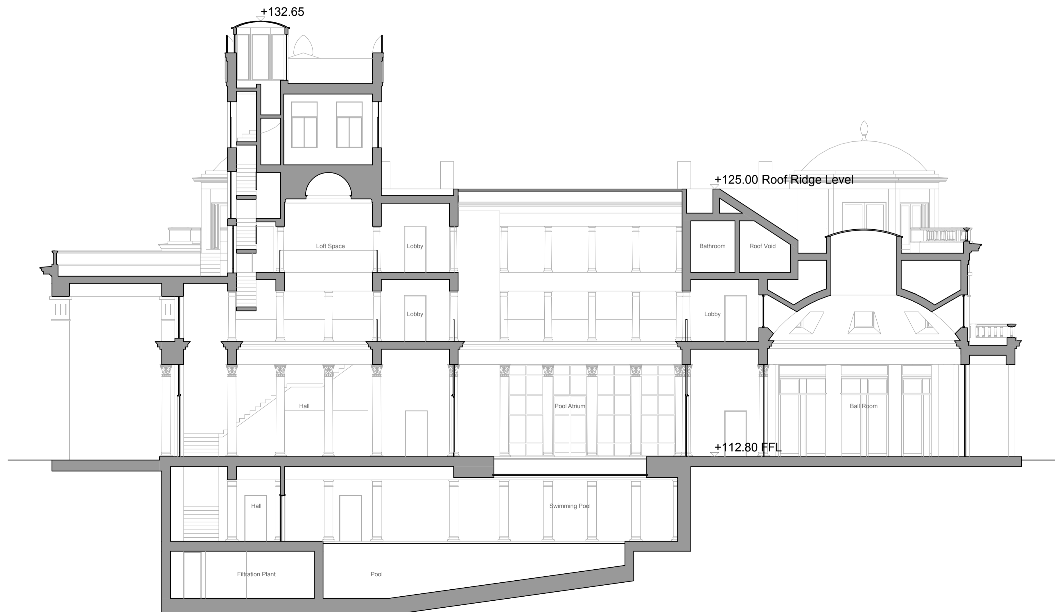
Section B-B
