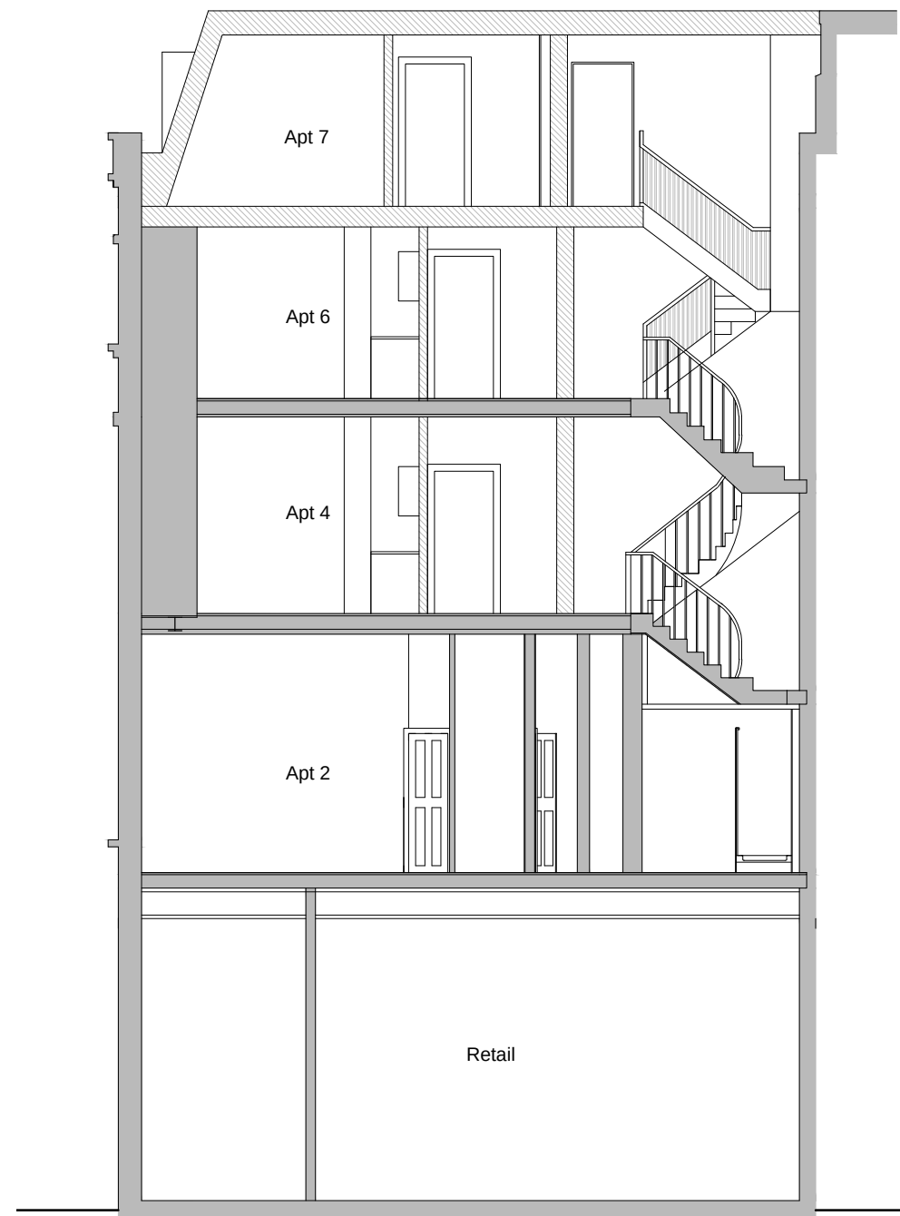
SECTION B-B
