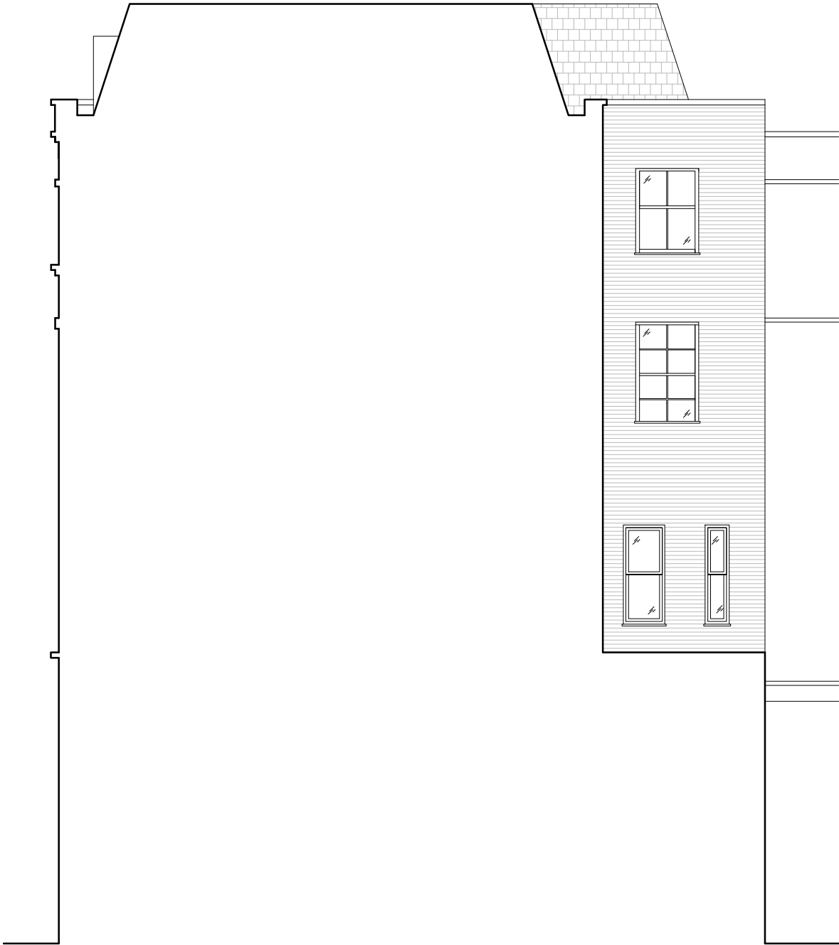
NORTH WEST ELEVATION
