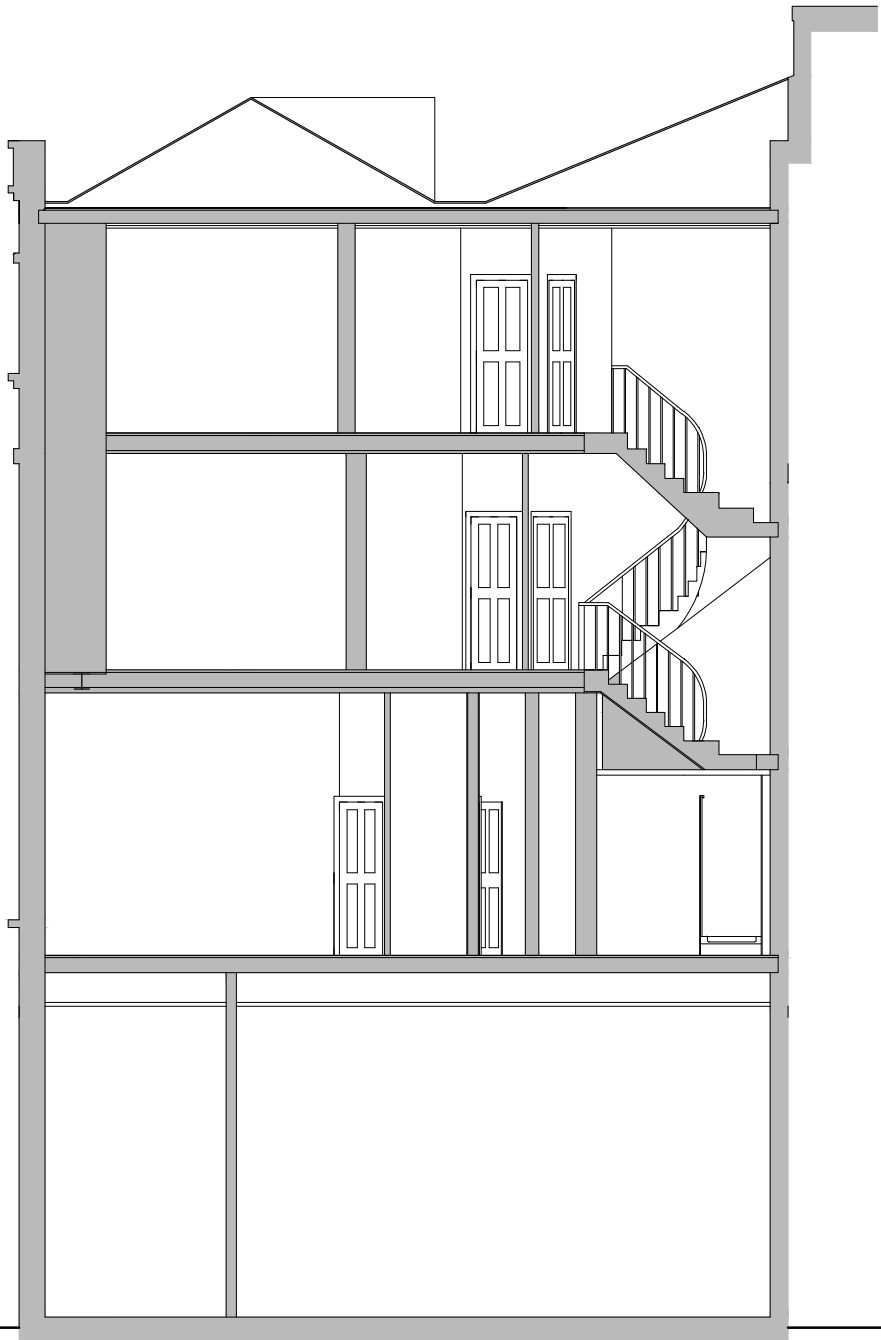
SECTION B-B
