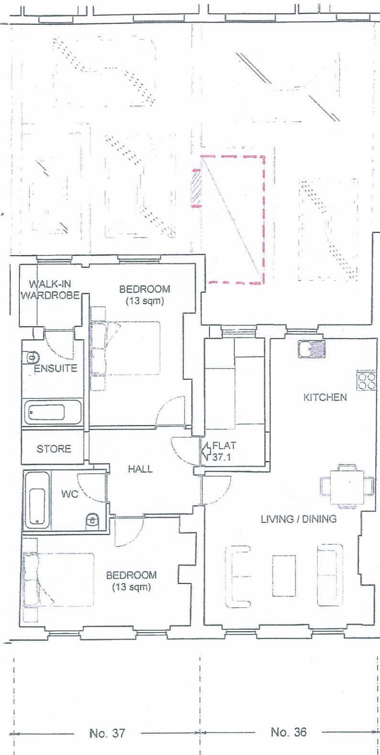
EXISTING FIRST FLOOR @ 1:100.
