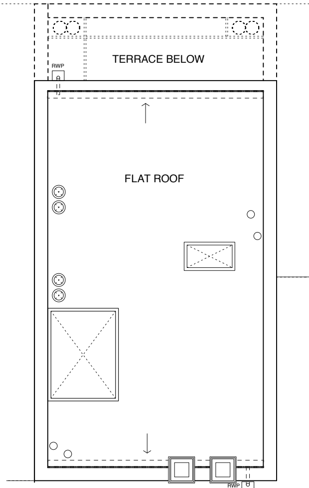
ROOF PLAN
