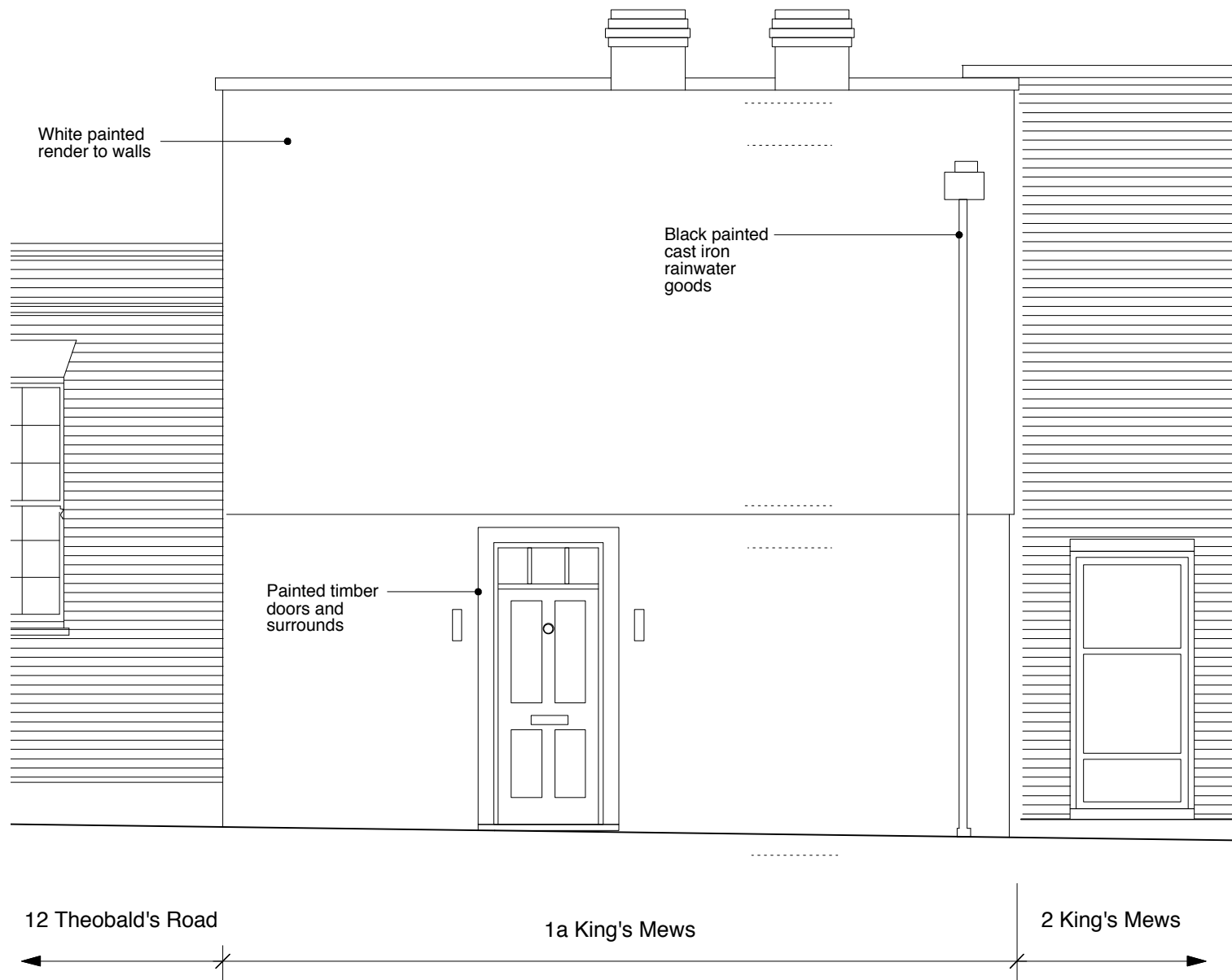
EXISTING EAST ELEVATION, HIGHLIGHTED SITE 1:50 @ A3
