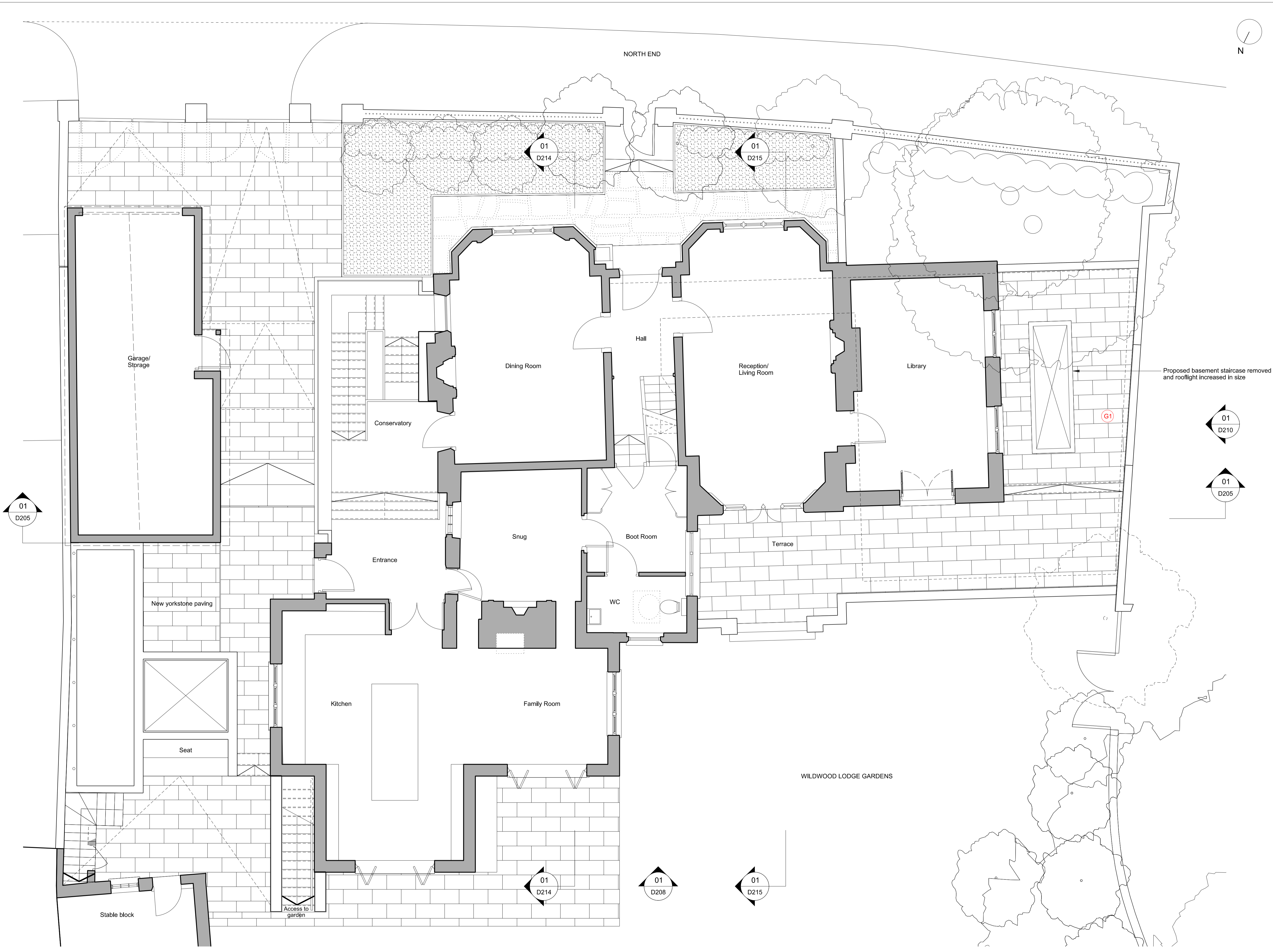
01 GROUND FLOOR PLAN D201 PROPOSED 1:50
