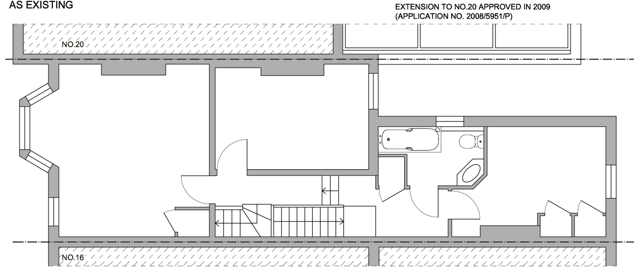
FIRST FLOOR PLAN AS EXISTING
