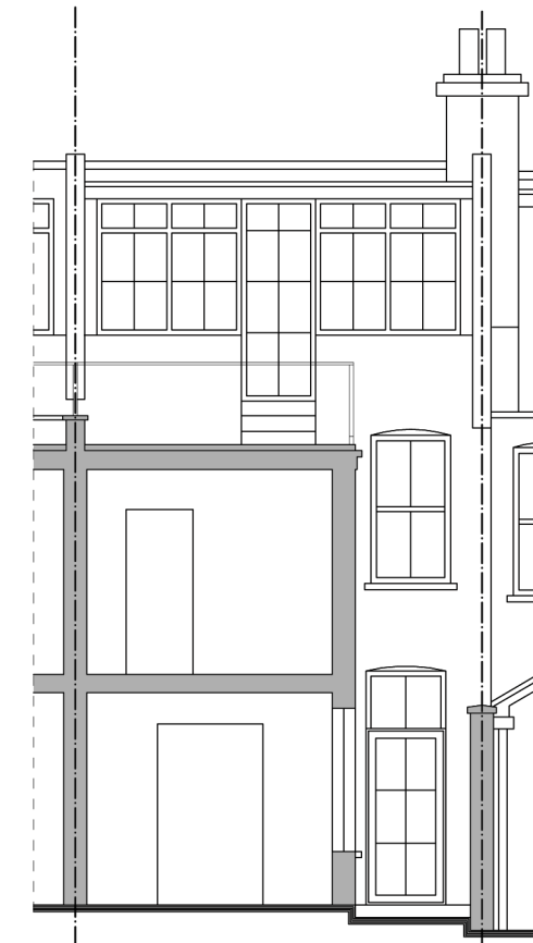
REAR ELEVATION / SECTION AS EXISTING
