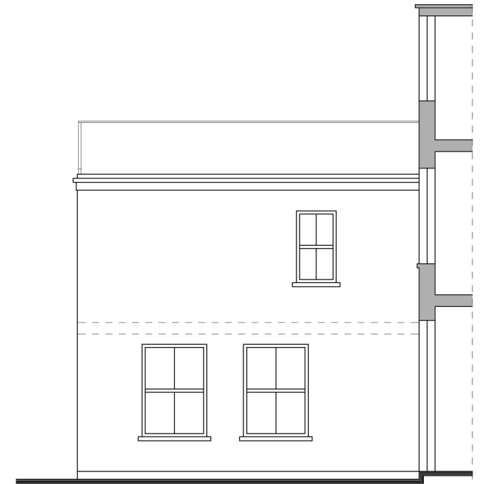
SIDE ELEVATION / SECTION AS EXISTING
