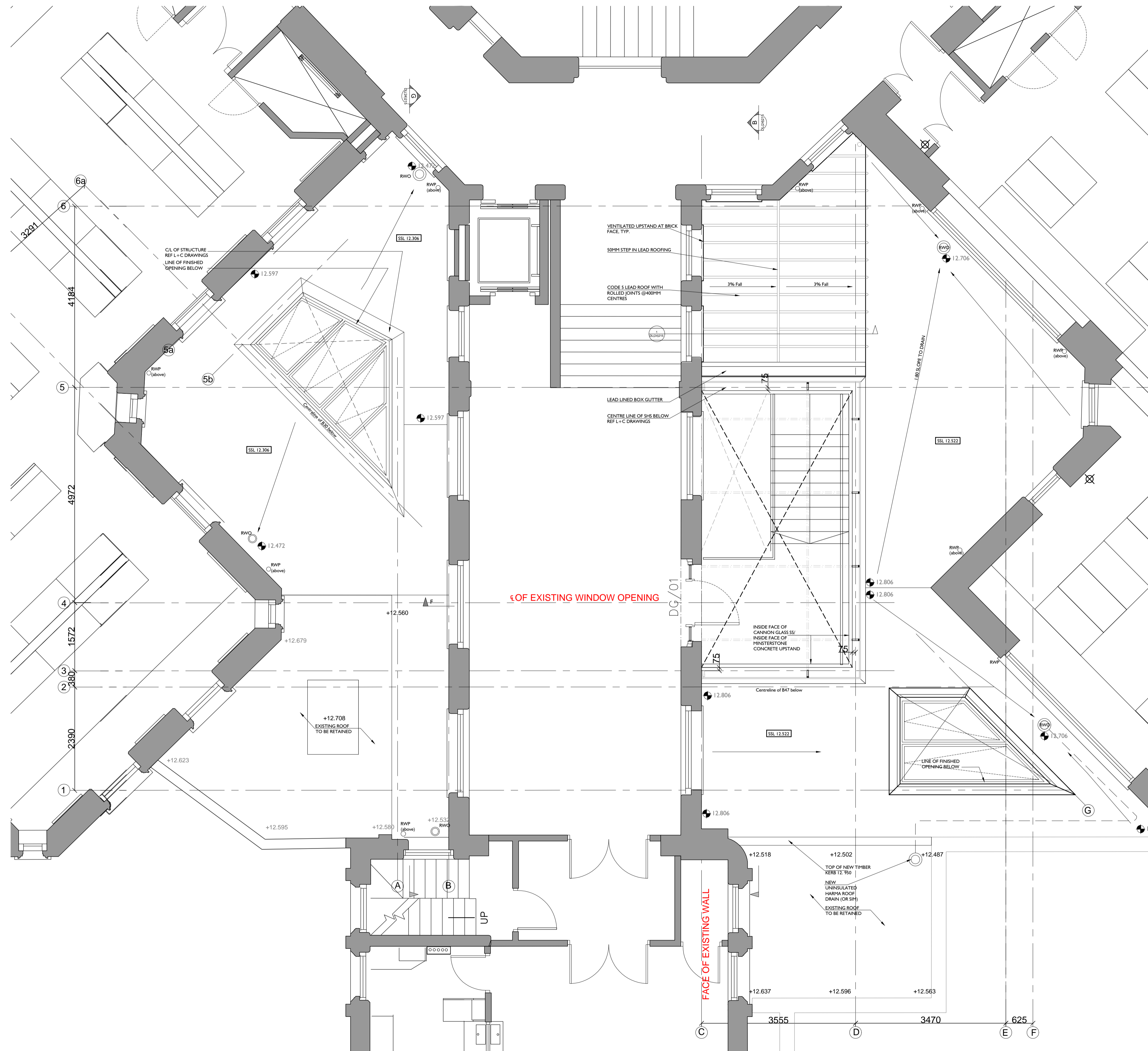
GROUND FLOOR/ROOF PLAN 1:50
