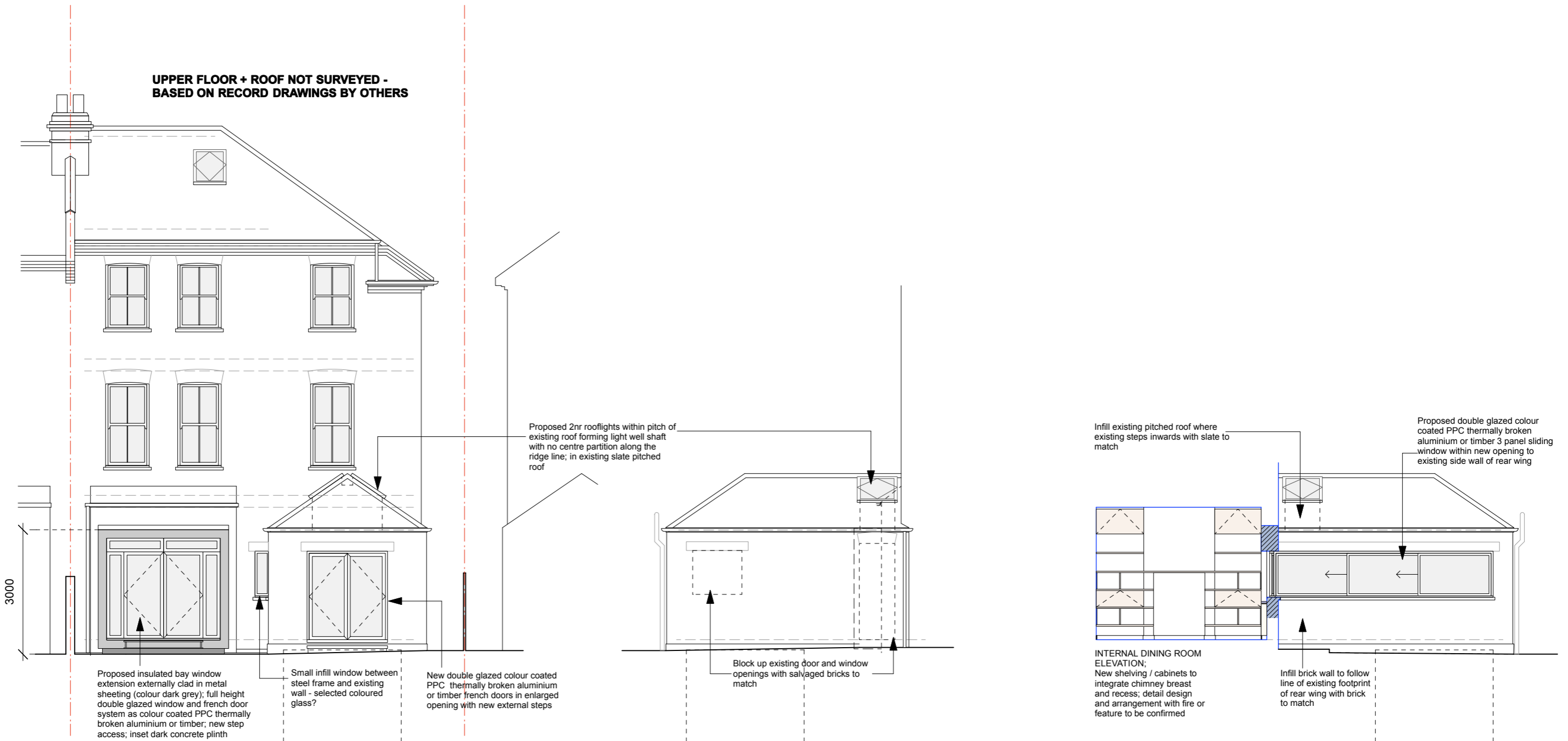
Rear Elevation : Proposed Scale 1:100
