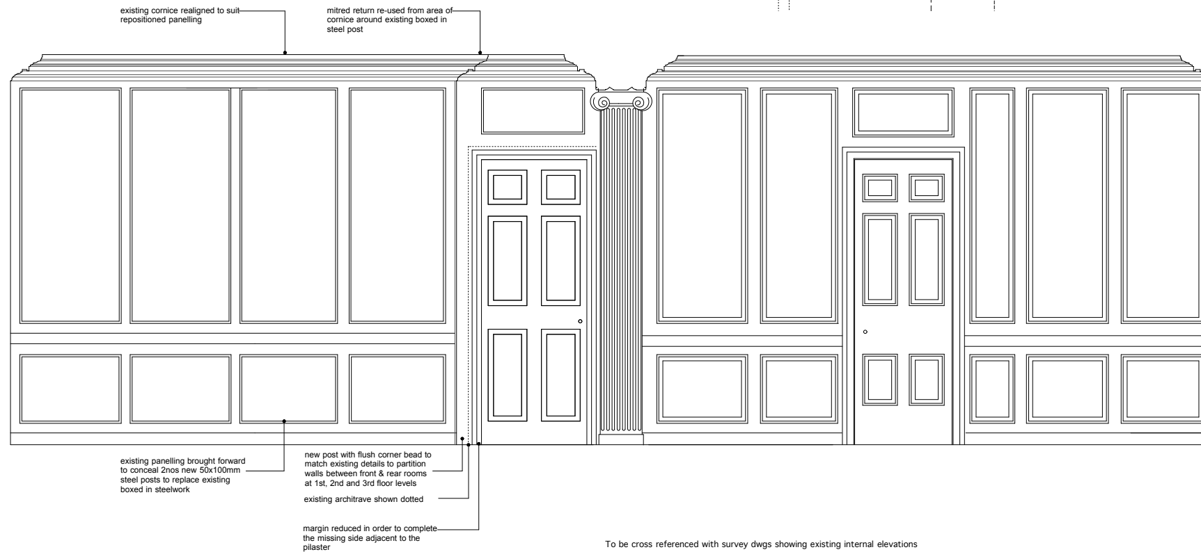
SECTION 01: GROUND FLOOR PANELLING Scale 1:20@ A1, 1:40@A3
