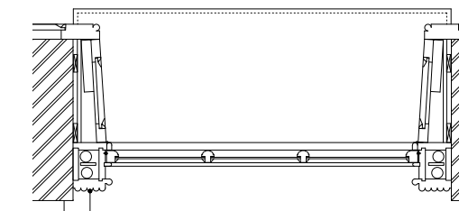
GROUND FLOOR WINDOWS: WG01 & WG02 PLAN DETAILS 04 (1:10@A1, 1:20@A3) existing box frame & architrave, new sashes with hw glazing bars, 4mm crown glass
