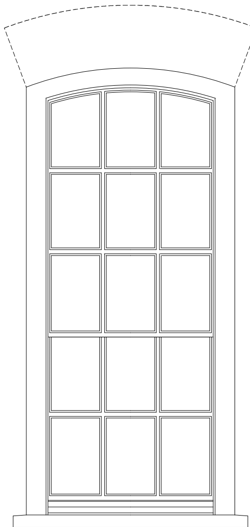
FIRST FLOOR: ELEVATION WF01, WF02, WF03 Scale 1:10@A1, 1:20@A3
