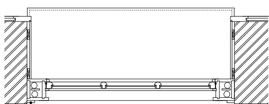
THIRD FLOOR WINDOWS: WT01, WT02, WT03 PLAN DETAILS 01 (1:10@A1, 1:20@A3) Glass Specification: 6.4mm Acoustic Glass
