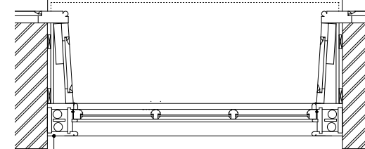
FIRST FLOOR WINDOWS: WF01, WF02, WF03 PLAN DETAILS 03 (1:10@A1, 1:20@A3) Glass Specification: 4mm Crown Glass
