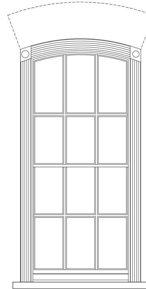
GROUND FLOOR: ELEVATION WG01, WG02, WG03 Scale 1:10@A1, 1:20@A3
