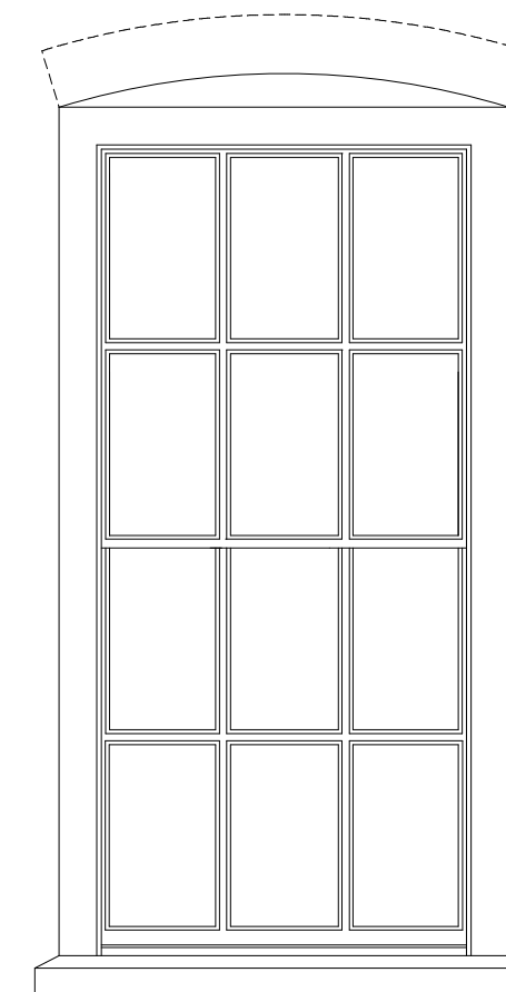
BASEMENT FLOOR: ELEVATION WB01, WB02 Scale 1:10@A1, 1:20@A3
