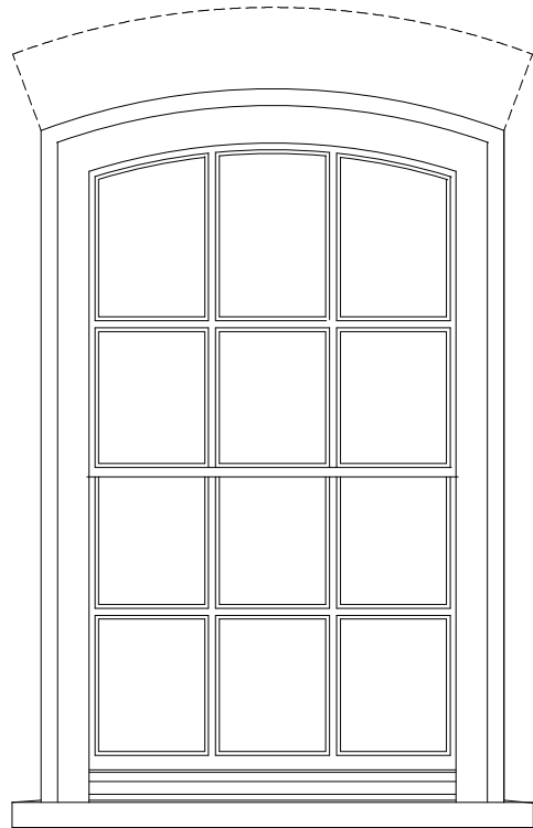
THIRD FLOOR: ELEVATION WT01, WT02, WT03 Scale 1:10@A1, 1:20@A3
