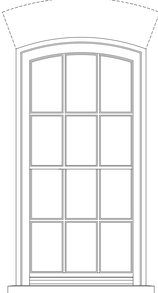
SECOND FLOOR: ELEVATION WS01, WS02, WS03 Scale 1:10@A1, 1:20@A3
