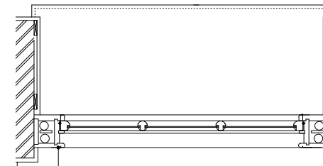
BASEMENT WINDOWS: WB01 & WB02 PLAN DETAILS 05 (1:10@A1, 1:20@A3) existing box frame fitted with new sashes, hw glazing bars, 6.4mm toughened glass
