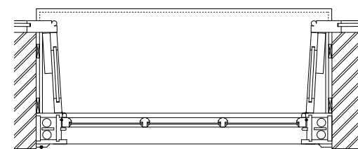
SECOND FLOOR WINDOWS: WS01, WS02, WS03 PLAN DETAILS 02 (1:10@A1, 1:20@A3) Glass Specification: 6.4mm Acoustic Glass
