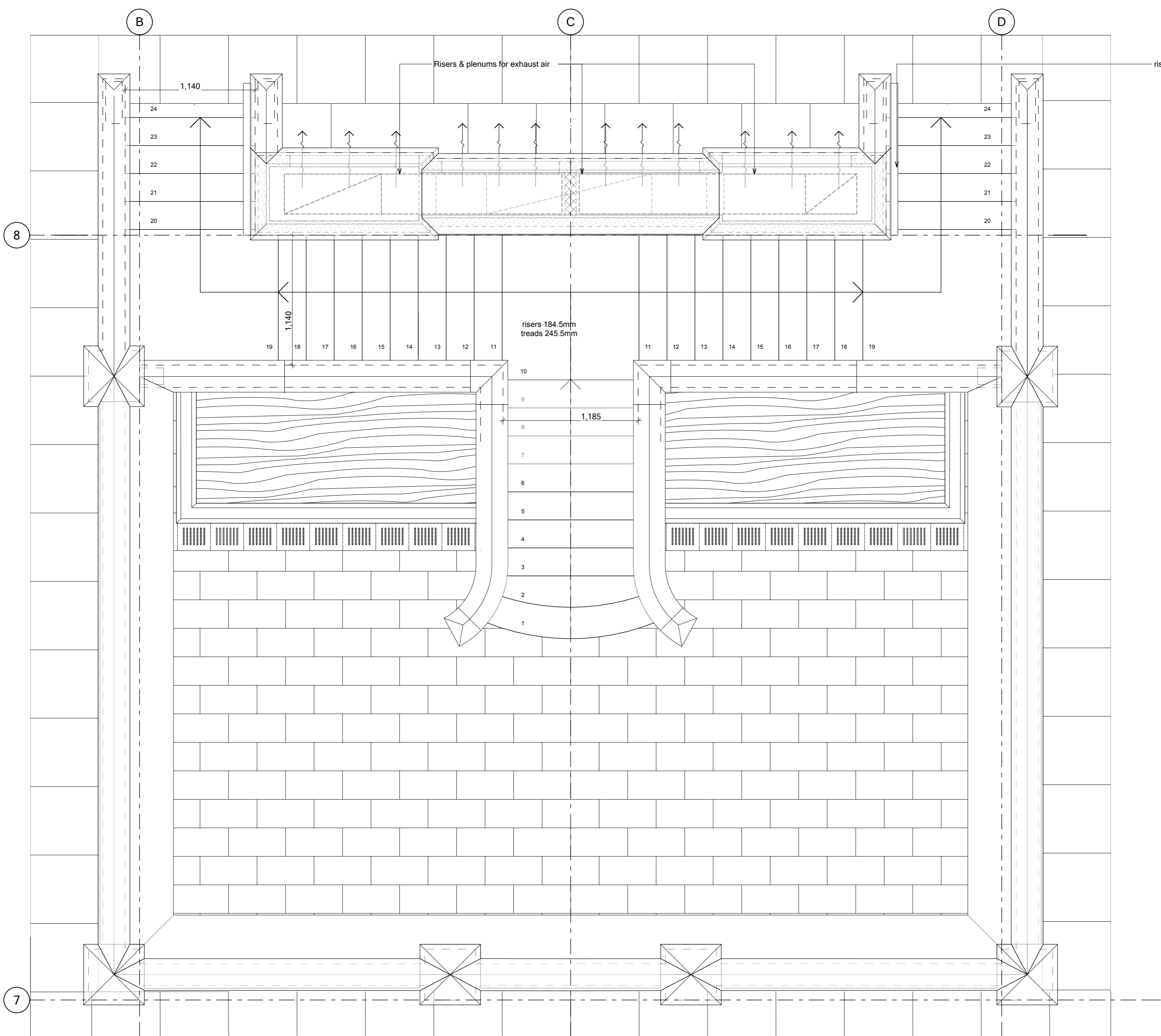
Courtyard GF Plan
