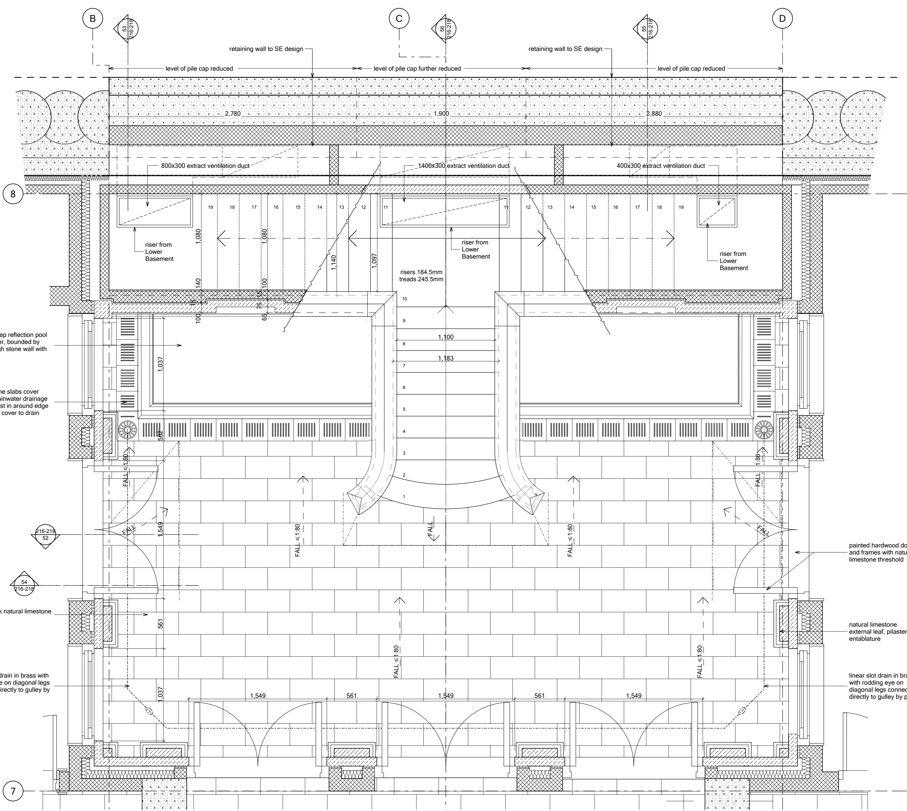
Courtyard UB Plan
