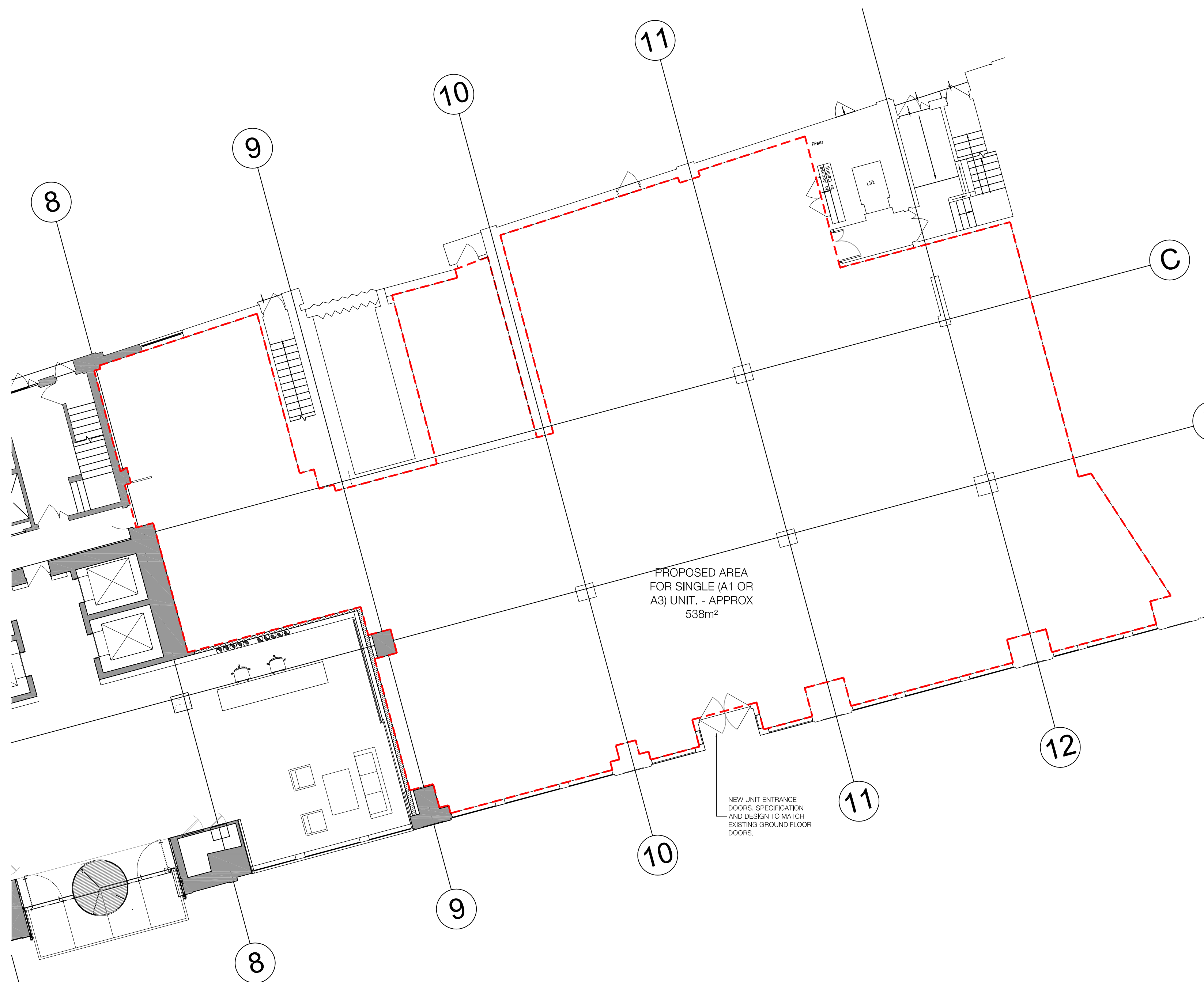
INDICATIVE LAYOUT - 1:100 @ A1
