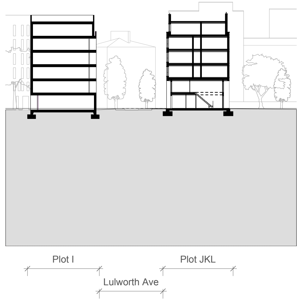
01 Proposed Site Section EE
