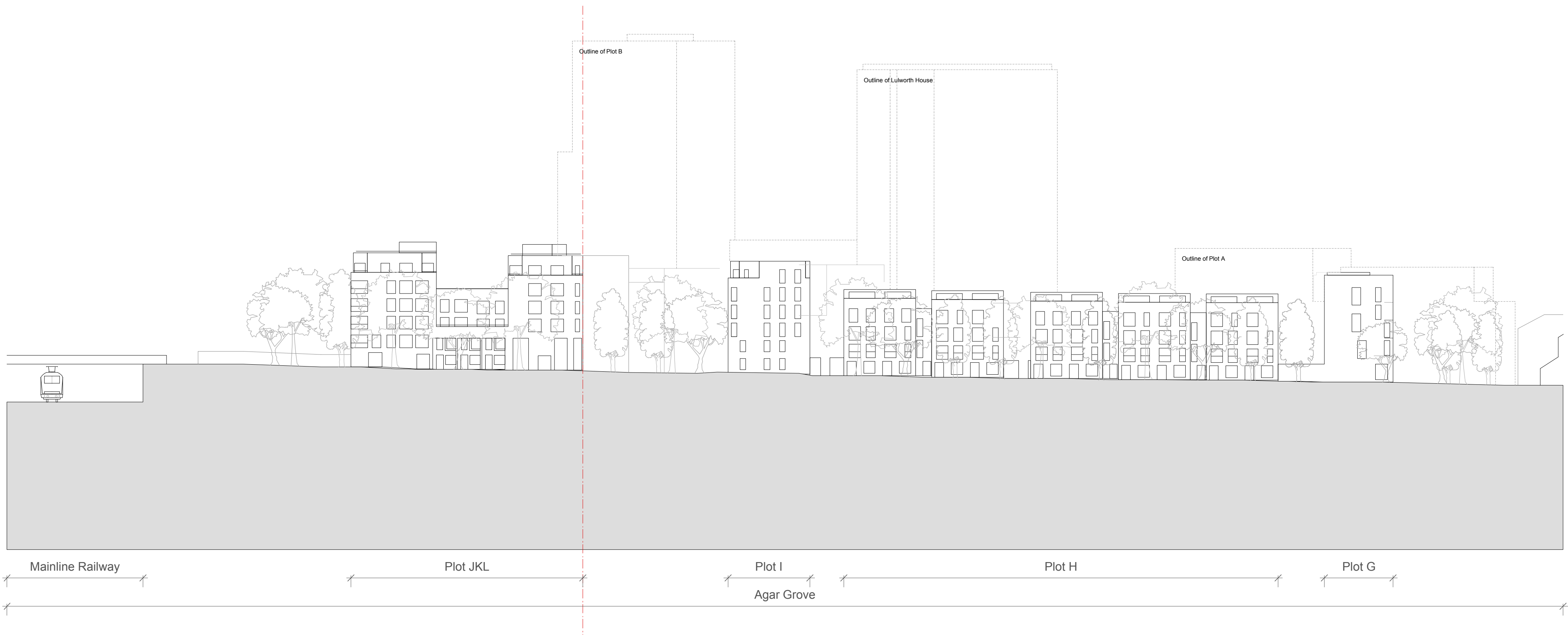
02 Proposed Site Section BB
