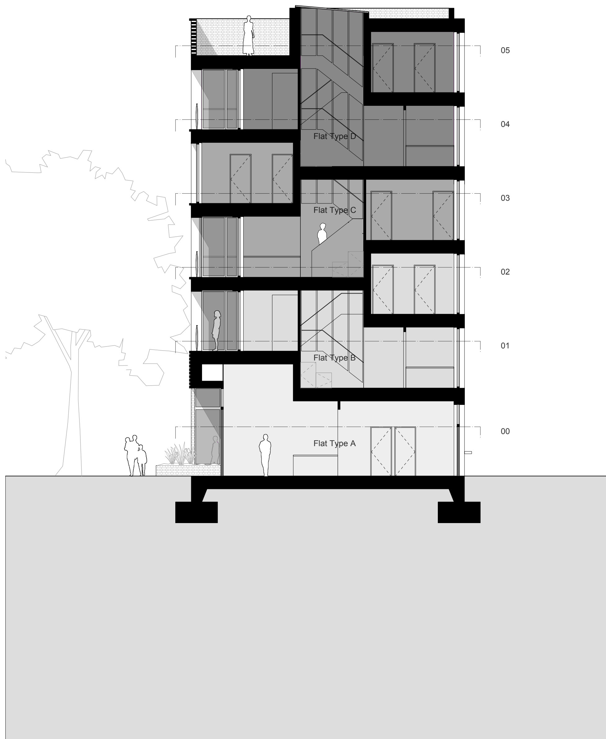
1 Block G Section BB 1:100
