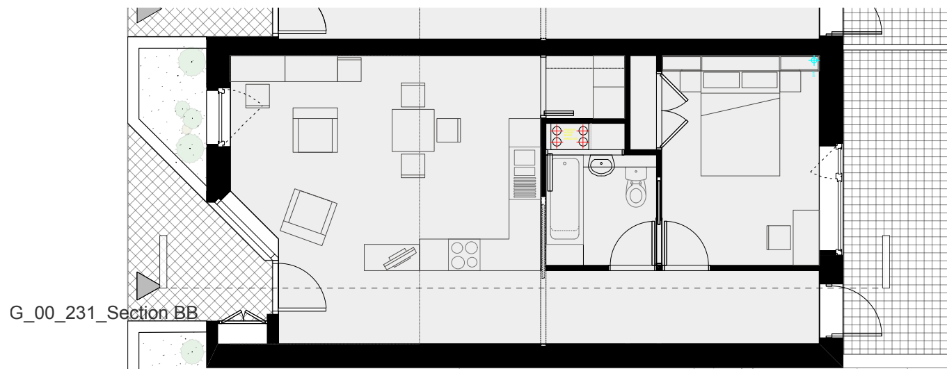
A Type A- Ground Floor Flat (1b 2p) 1:100
