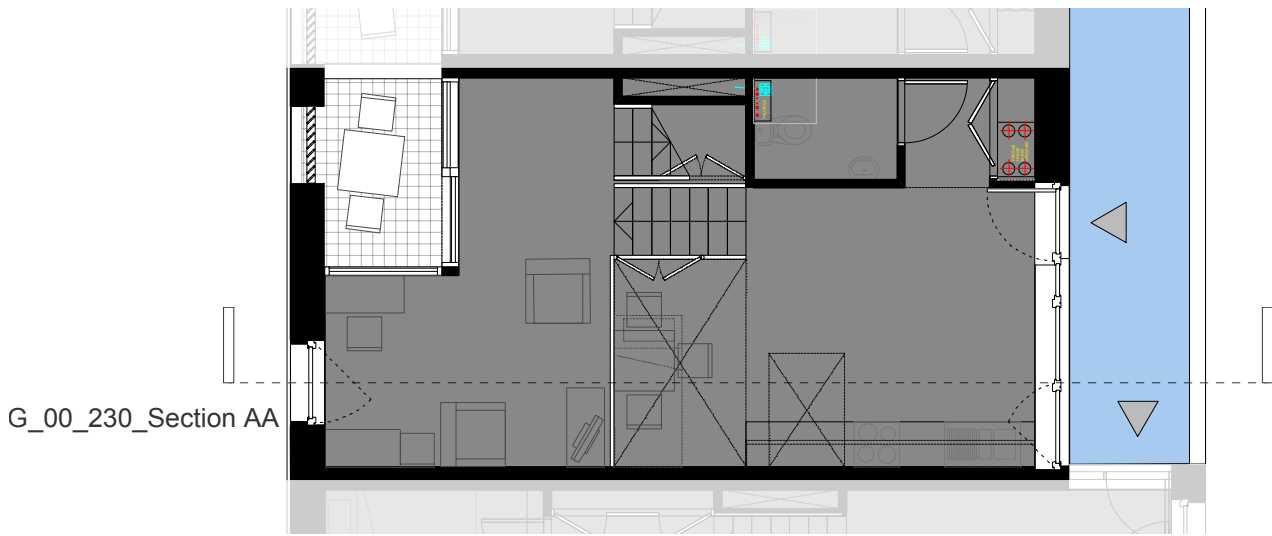
D Type D- Fourth Floor Entry Split-Level Flat (1b2p) 1:100
