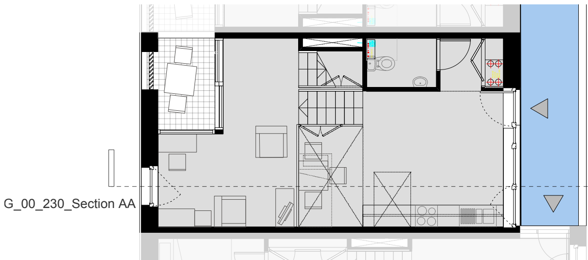
B Type B- First Floor Entry Split-Level Flat (1b2p) 1:100
