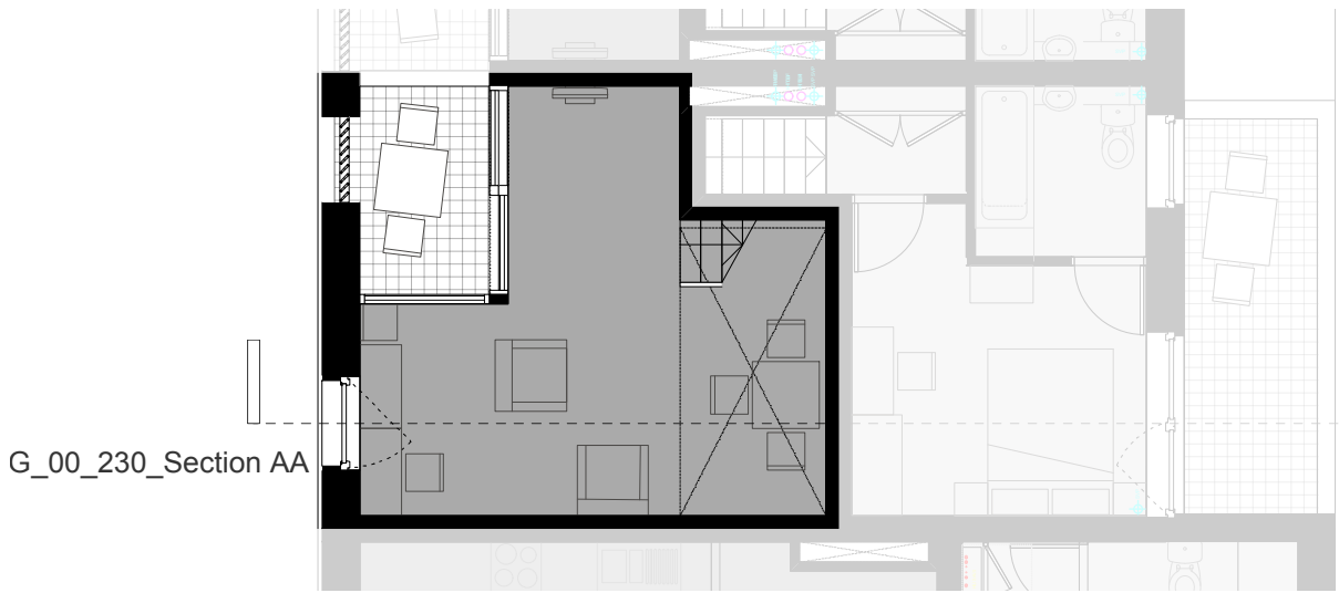
C Type C- Third Floor Entry Split-Level Flat (1b2p) 1:100
