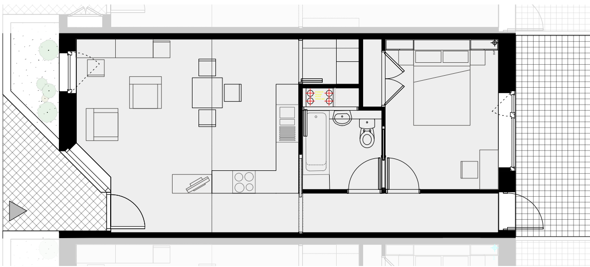
A Type A- Ground Floor Flat (1b2p) 1:100
