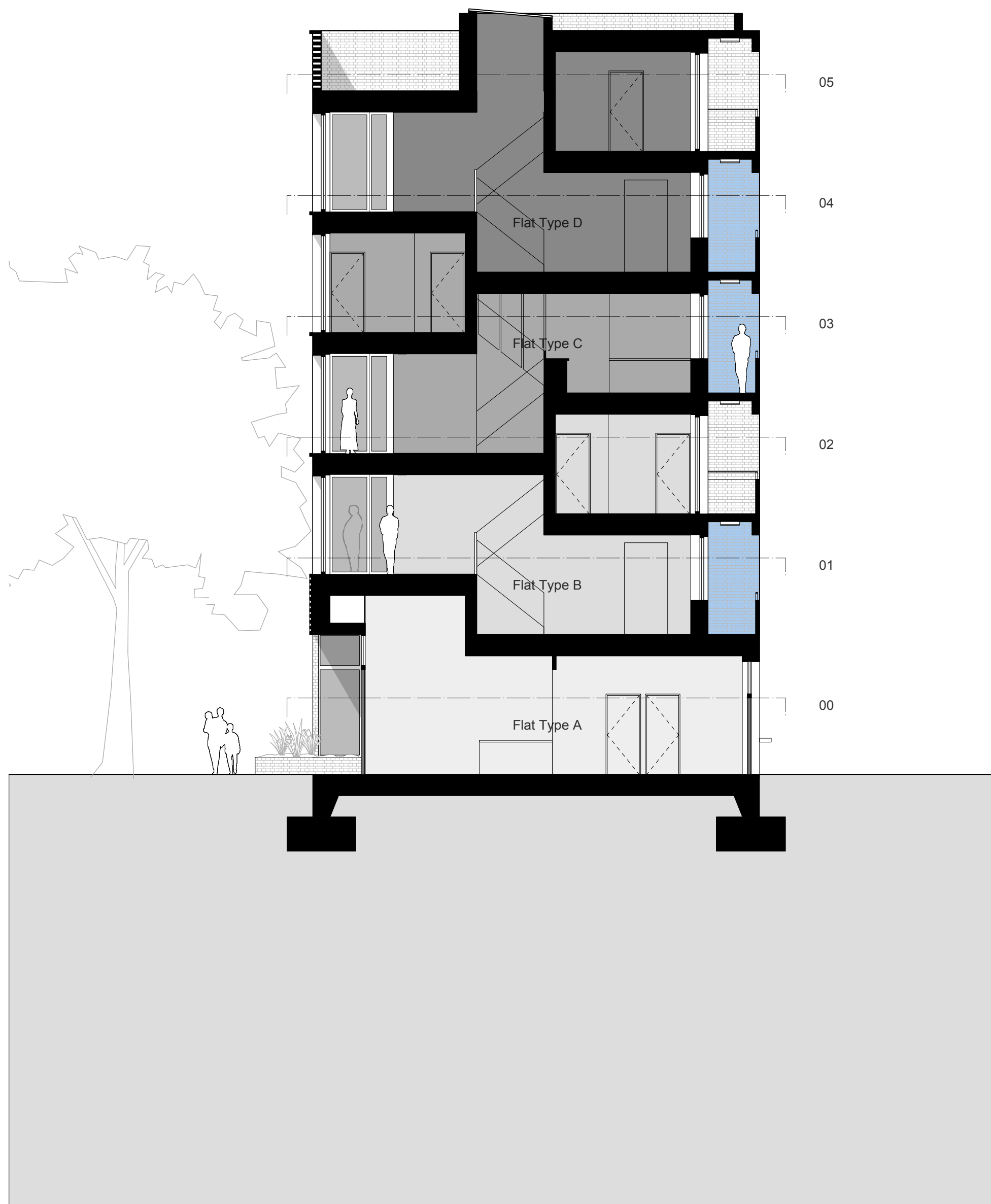
1 Block G Section AA 1:100
