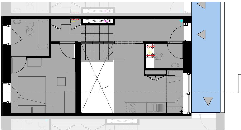
G_00_230_Section AA
