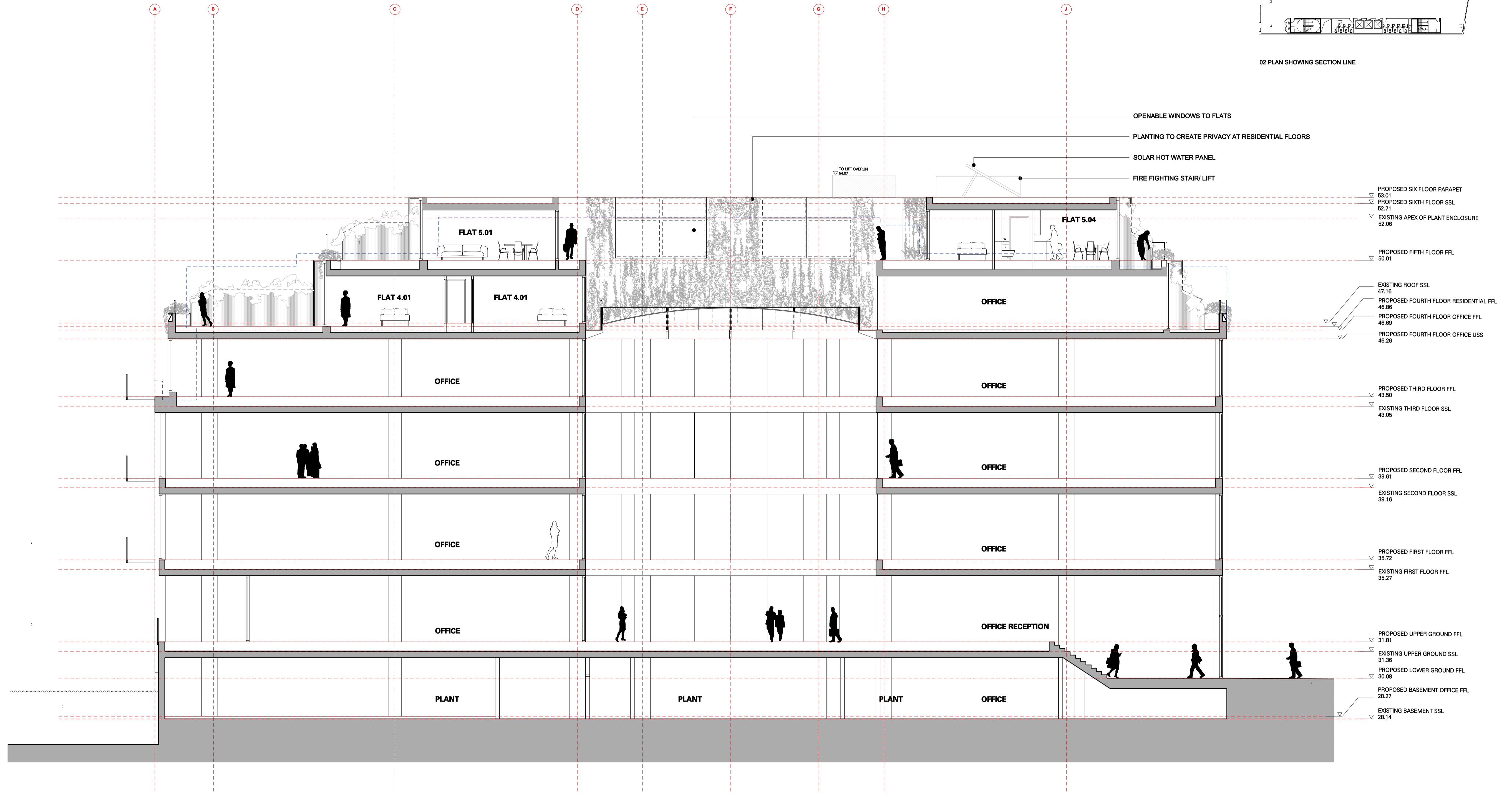
Sec 01 Proposed section AA Scale 1:100
