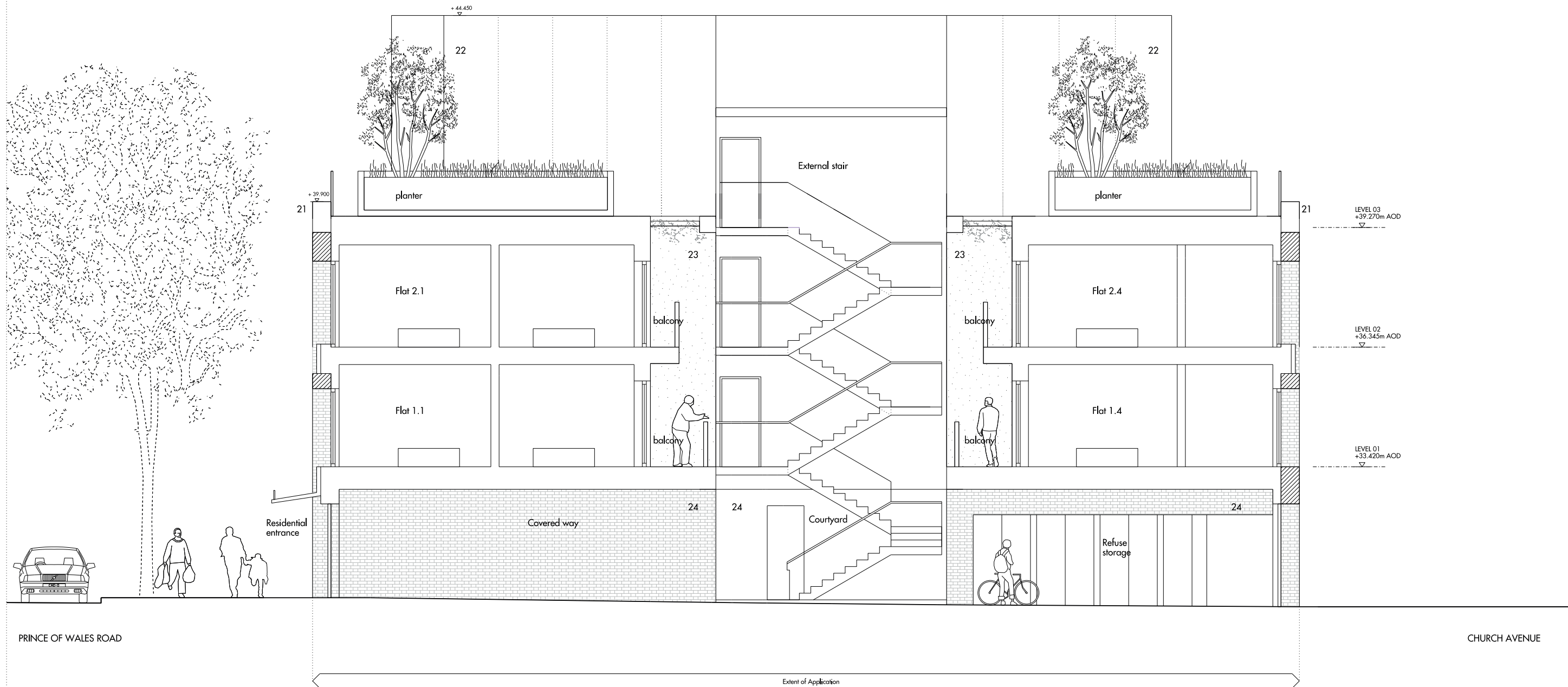
01 SECTION B - B SCALE 1:50 @ A1
