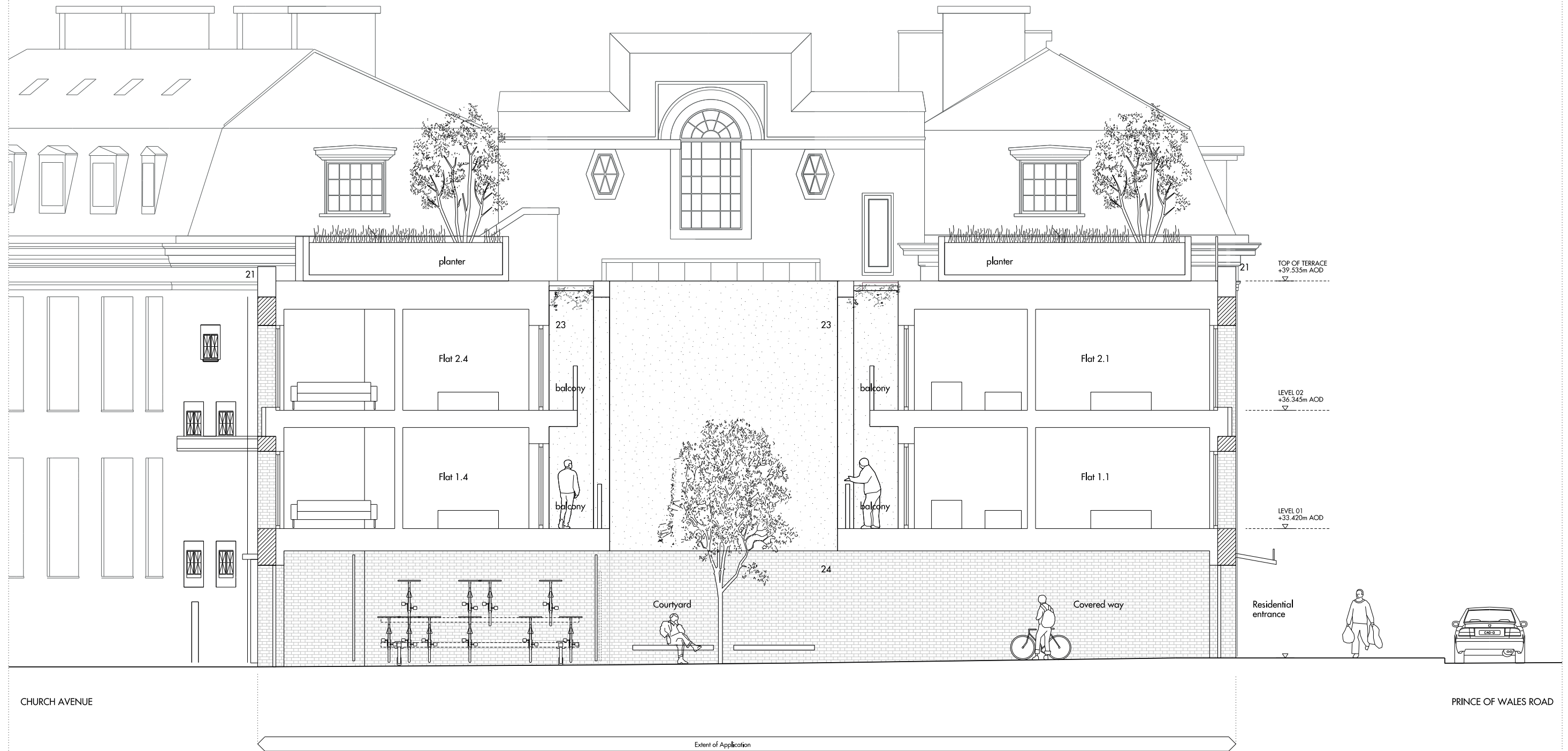
01 SECTION A - A SCALE 1:50 @ A1
