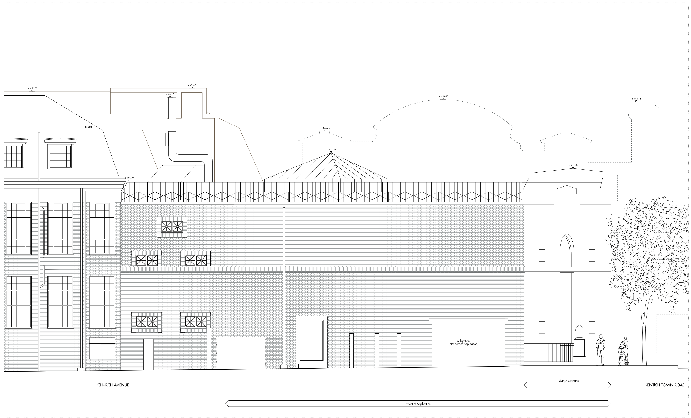
01 SOUTH ELEVATION SCALE 1:50 @ A1
