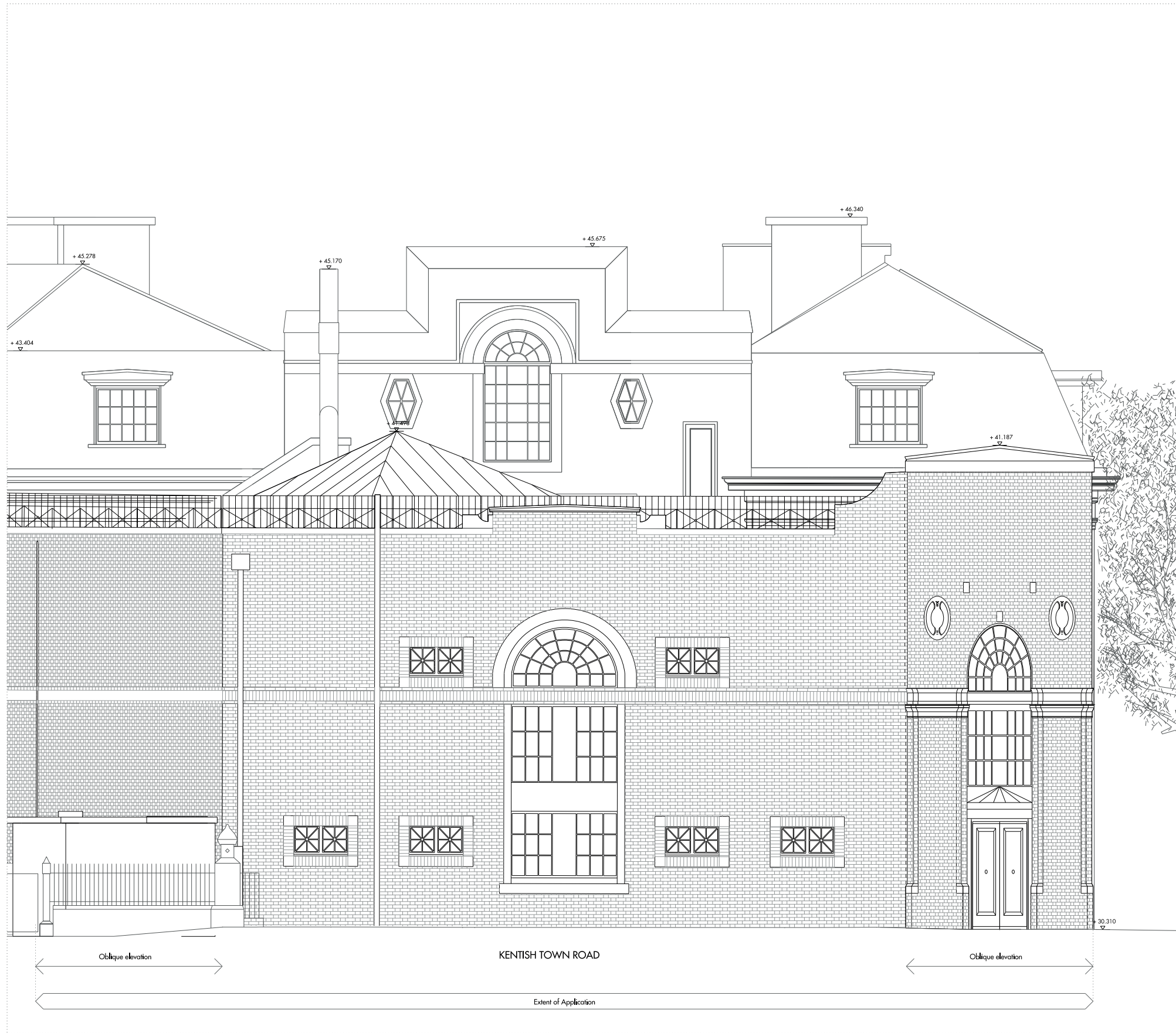
01 EAST ELEVATION SCALE 1:50 @ A1
