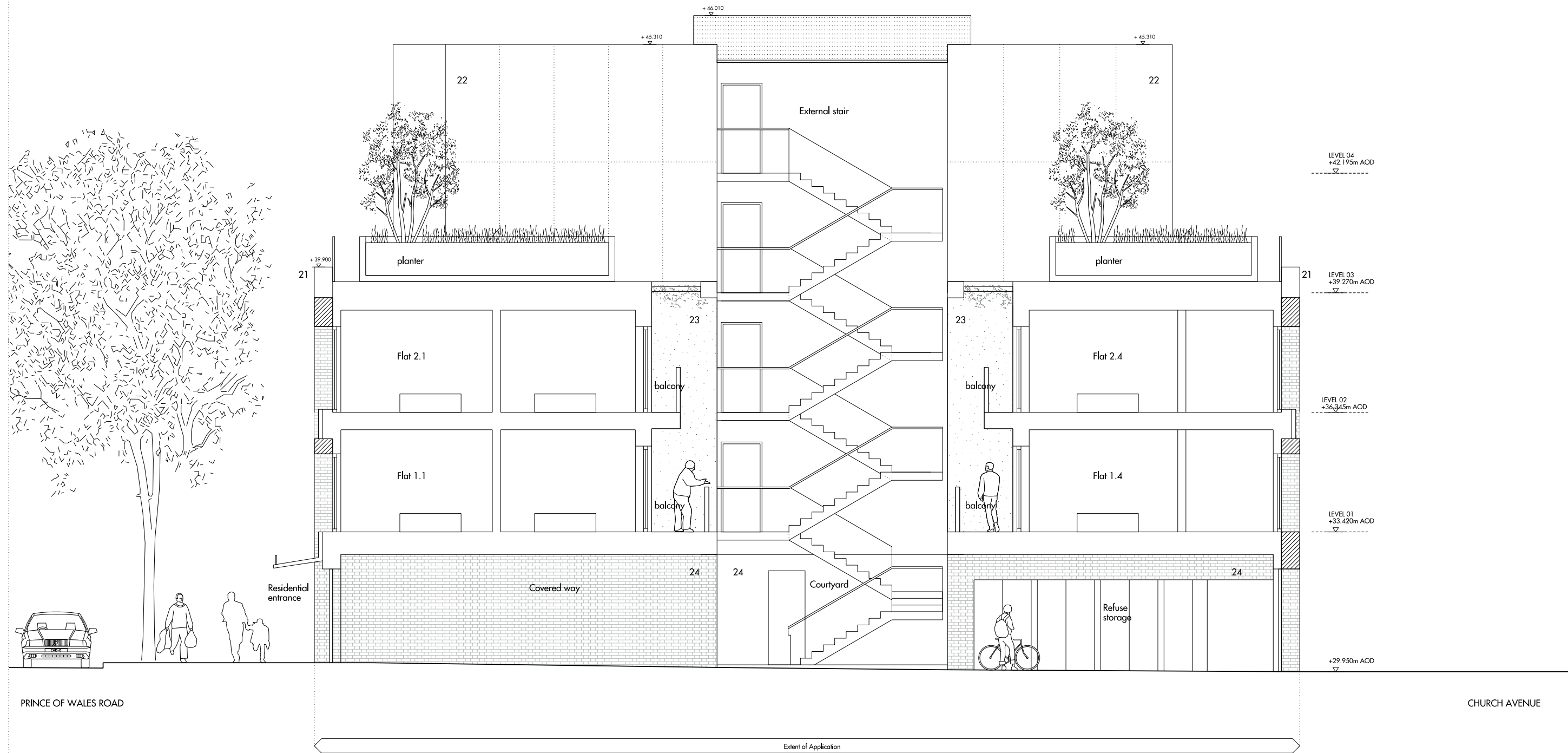
01 SECTION B - B SCALE 1:50 @ A1
