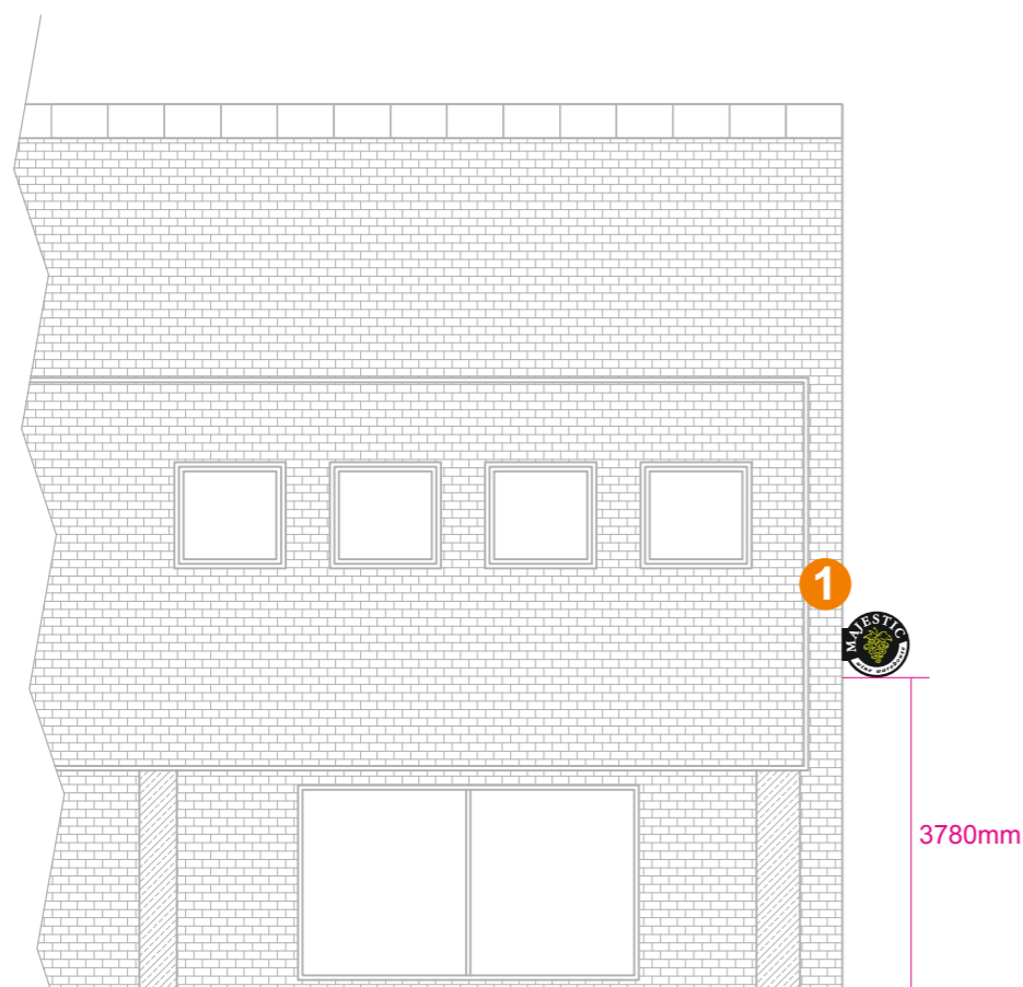
SIDE ELEVATION (SHELTON ST)
