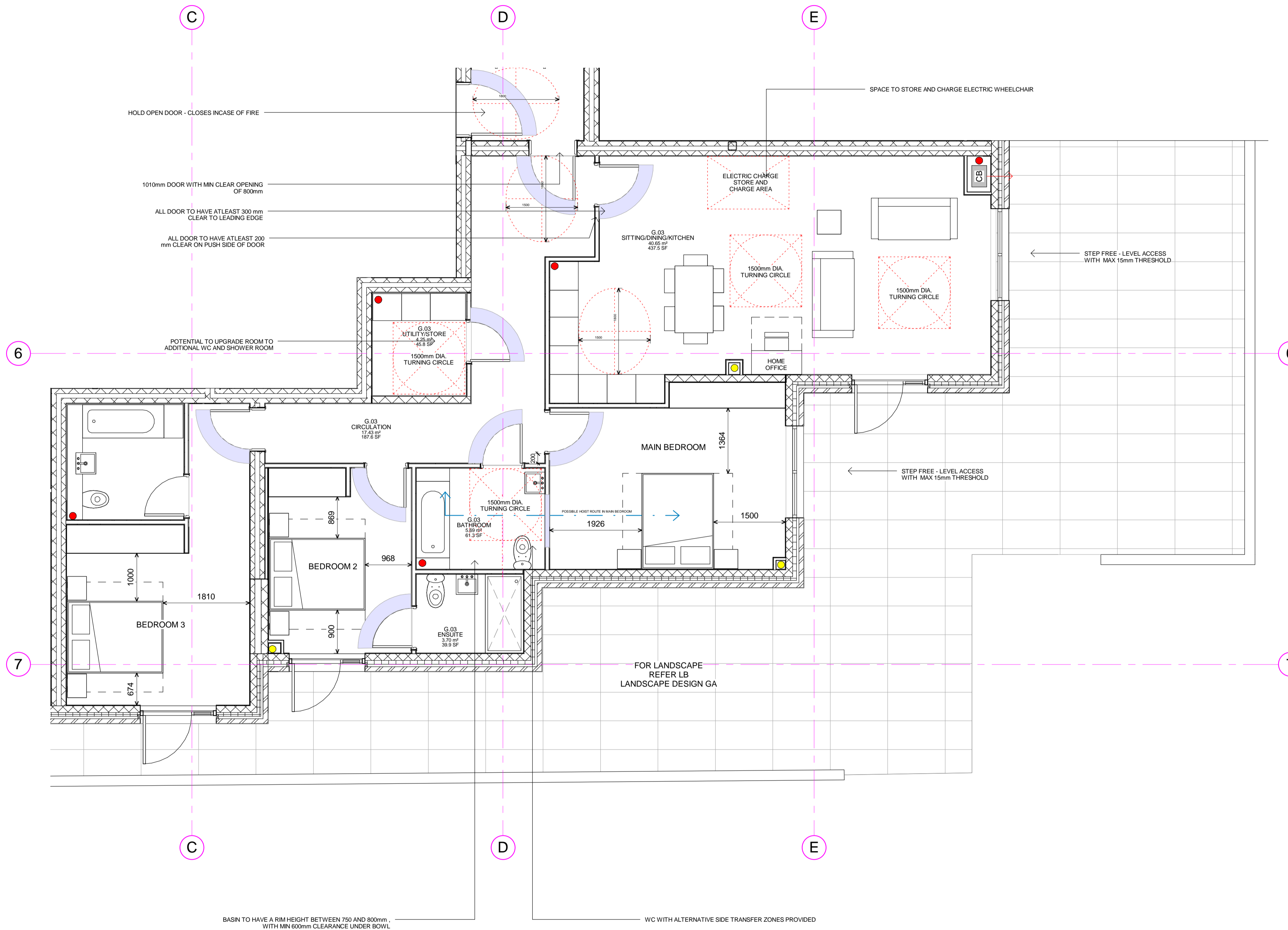
1 G.03 - WHEEL CHAIR ACCESSIBLE APARTMENT 1 : 50
