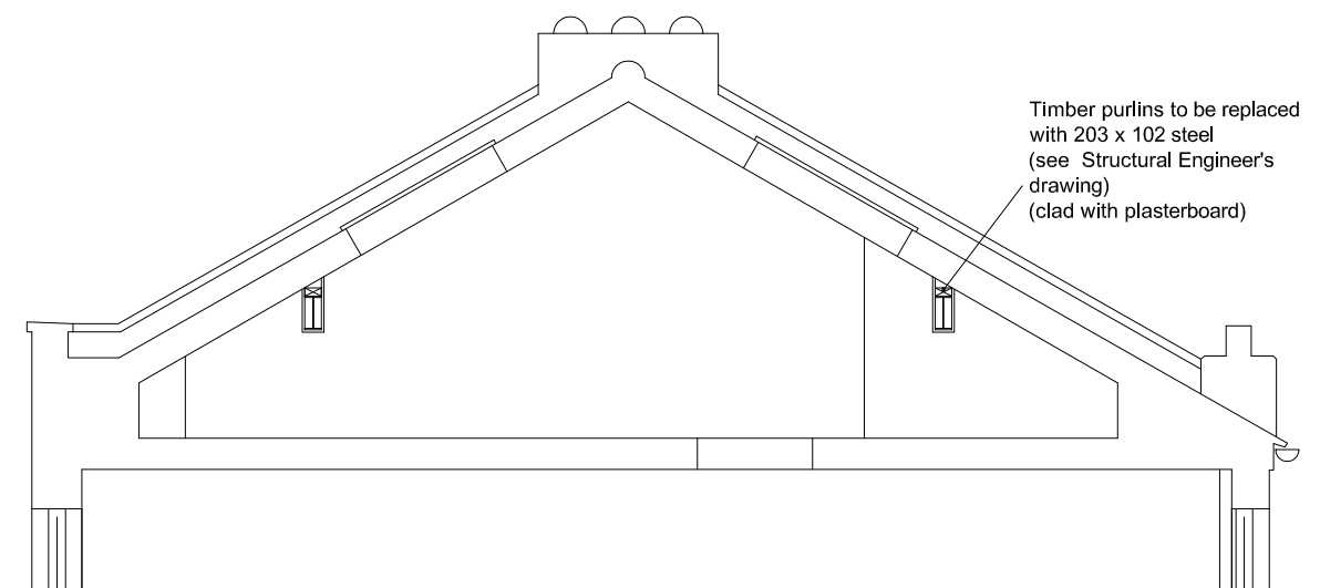
SECTION A-A AS PROPOSED
