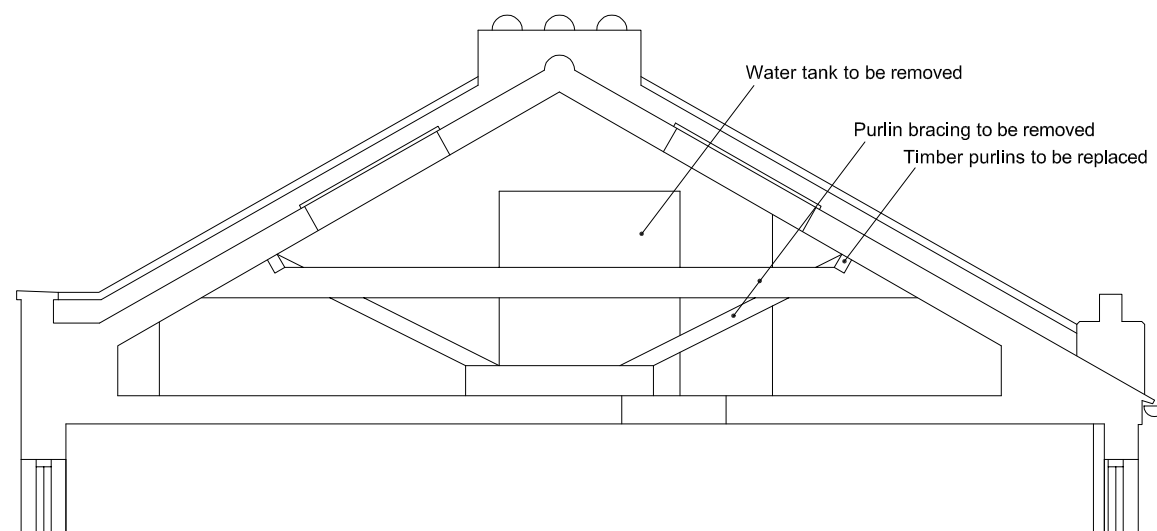
SECTION A-A AS EXISTING
