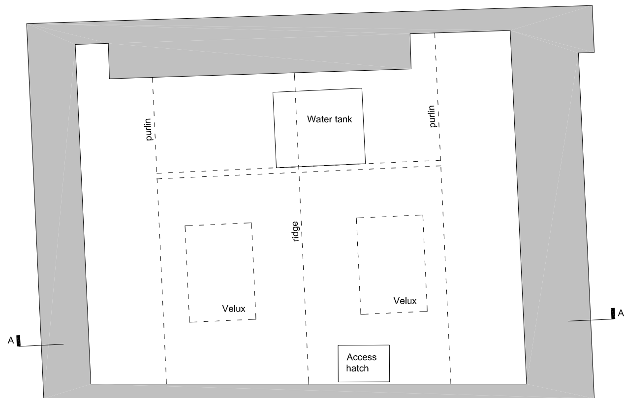
LOFT PLAN AS EXISTING
