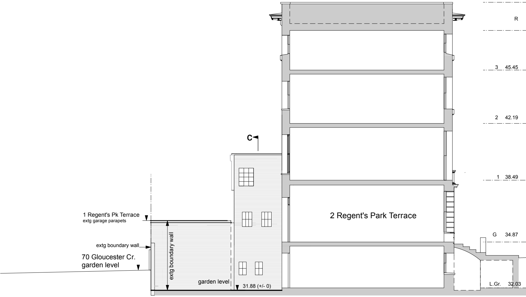
section D - D (1107-X-07)
