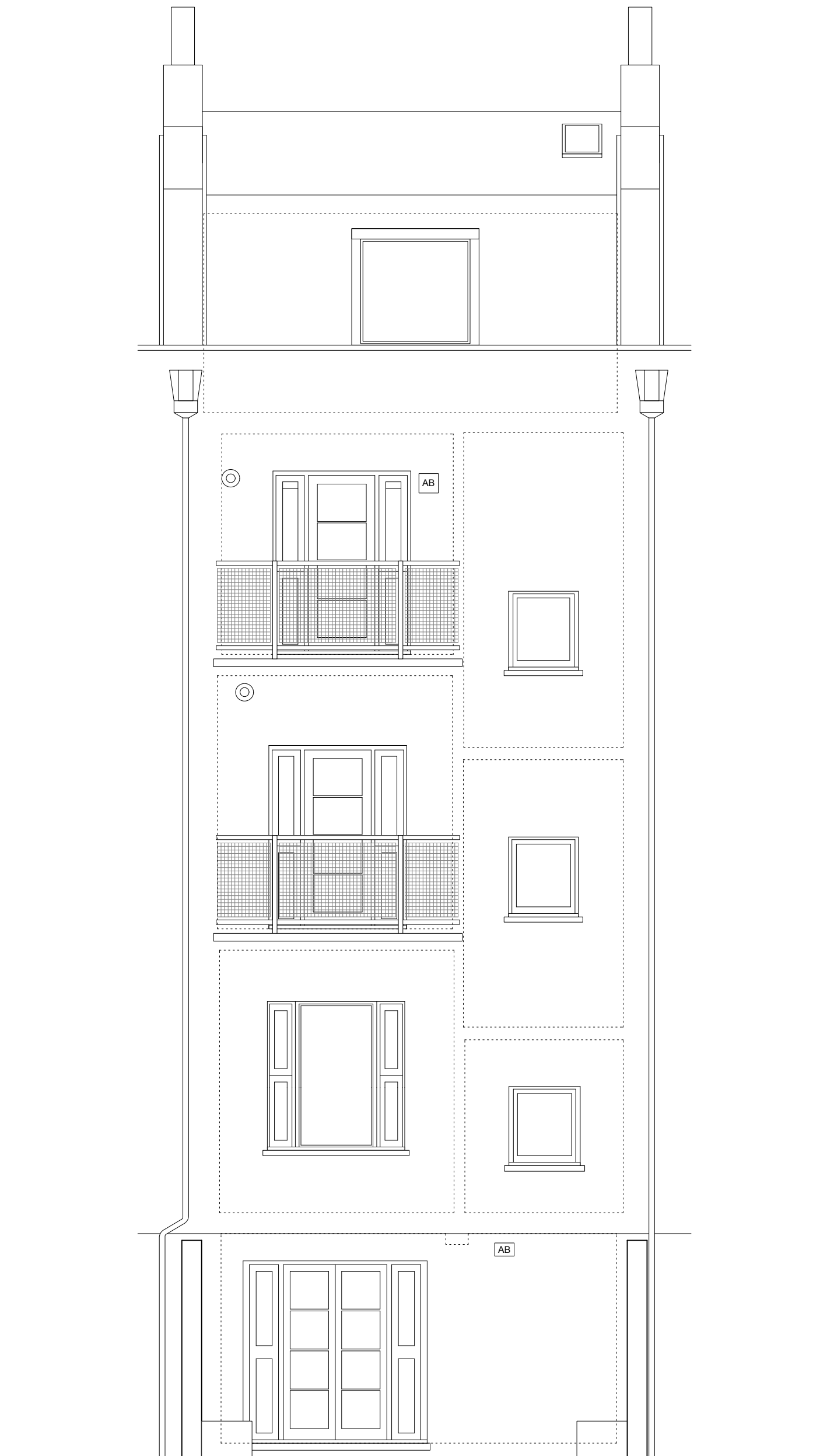
REAR ELEVATION
