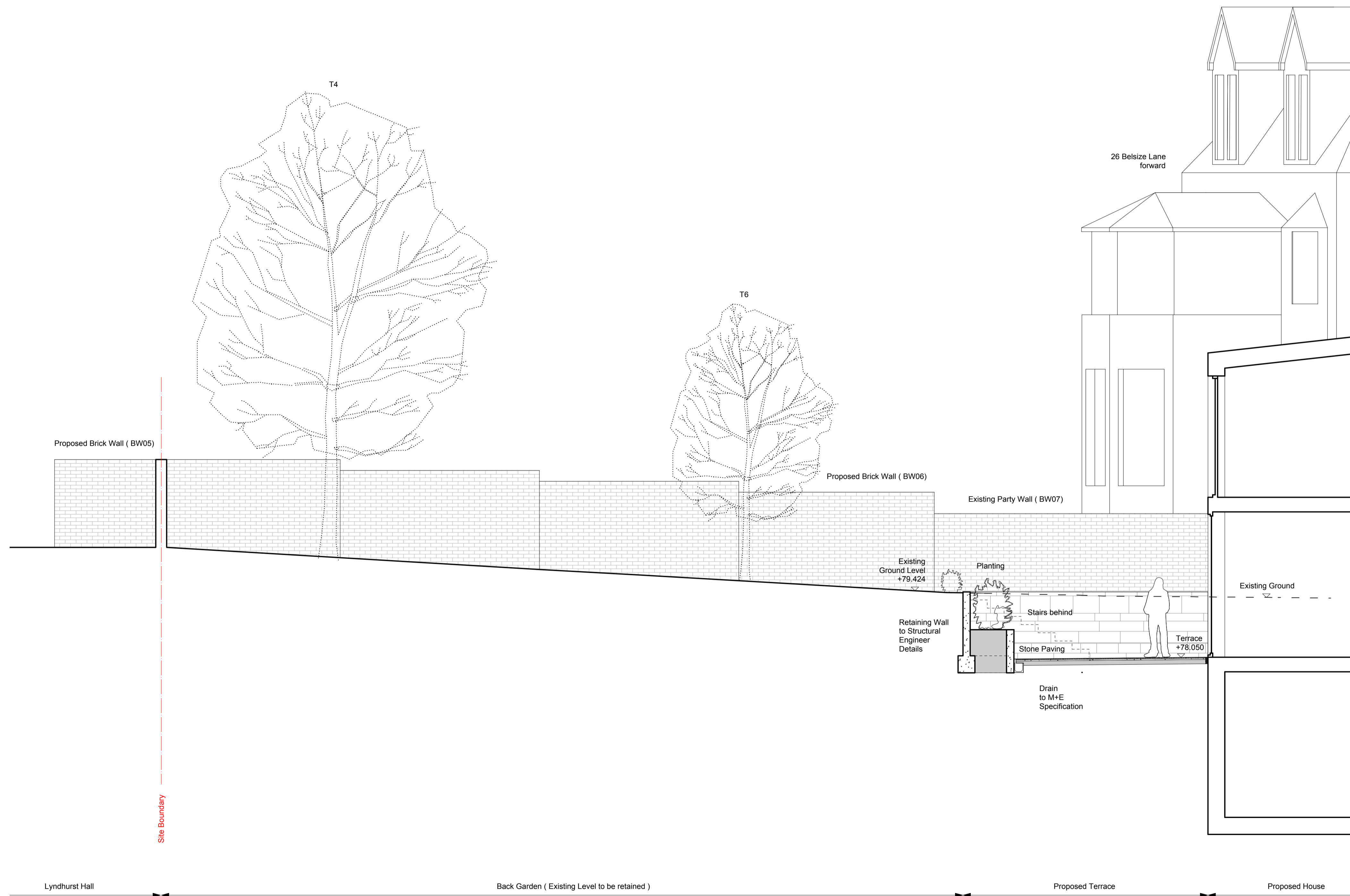
01 South Section Landscape Section Detail 1:50(A1)
