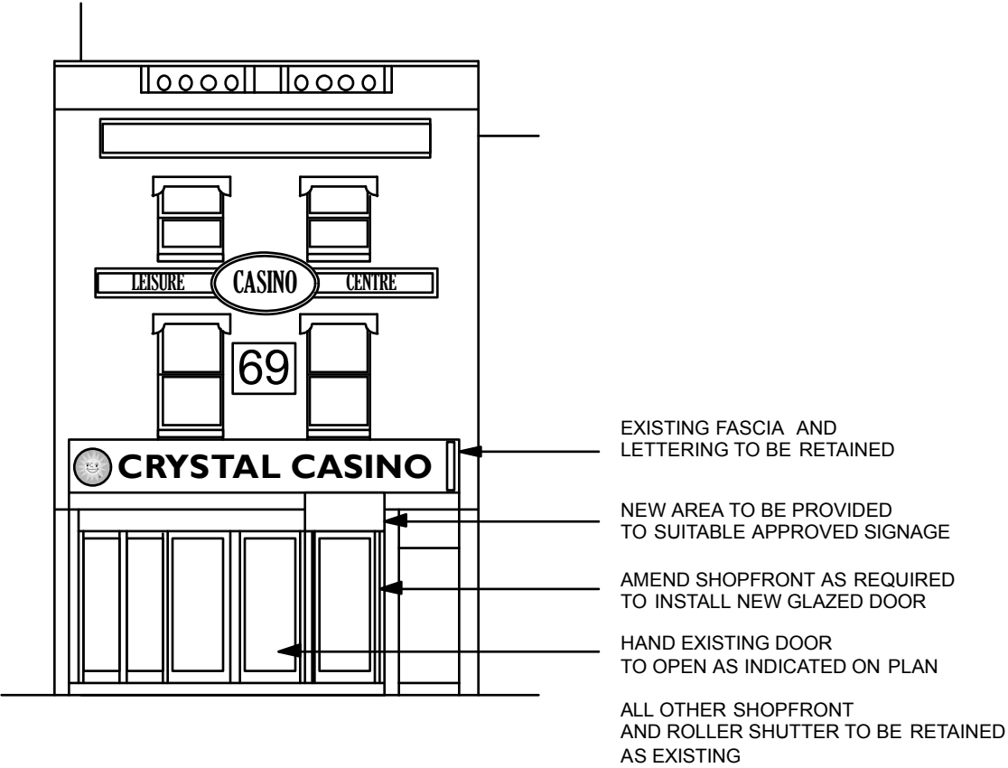
8 PROPOSED ELEVATION
