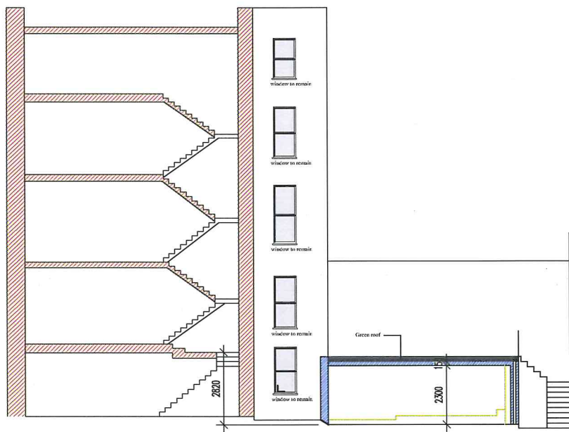
Proposed Side Elevation & Section
