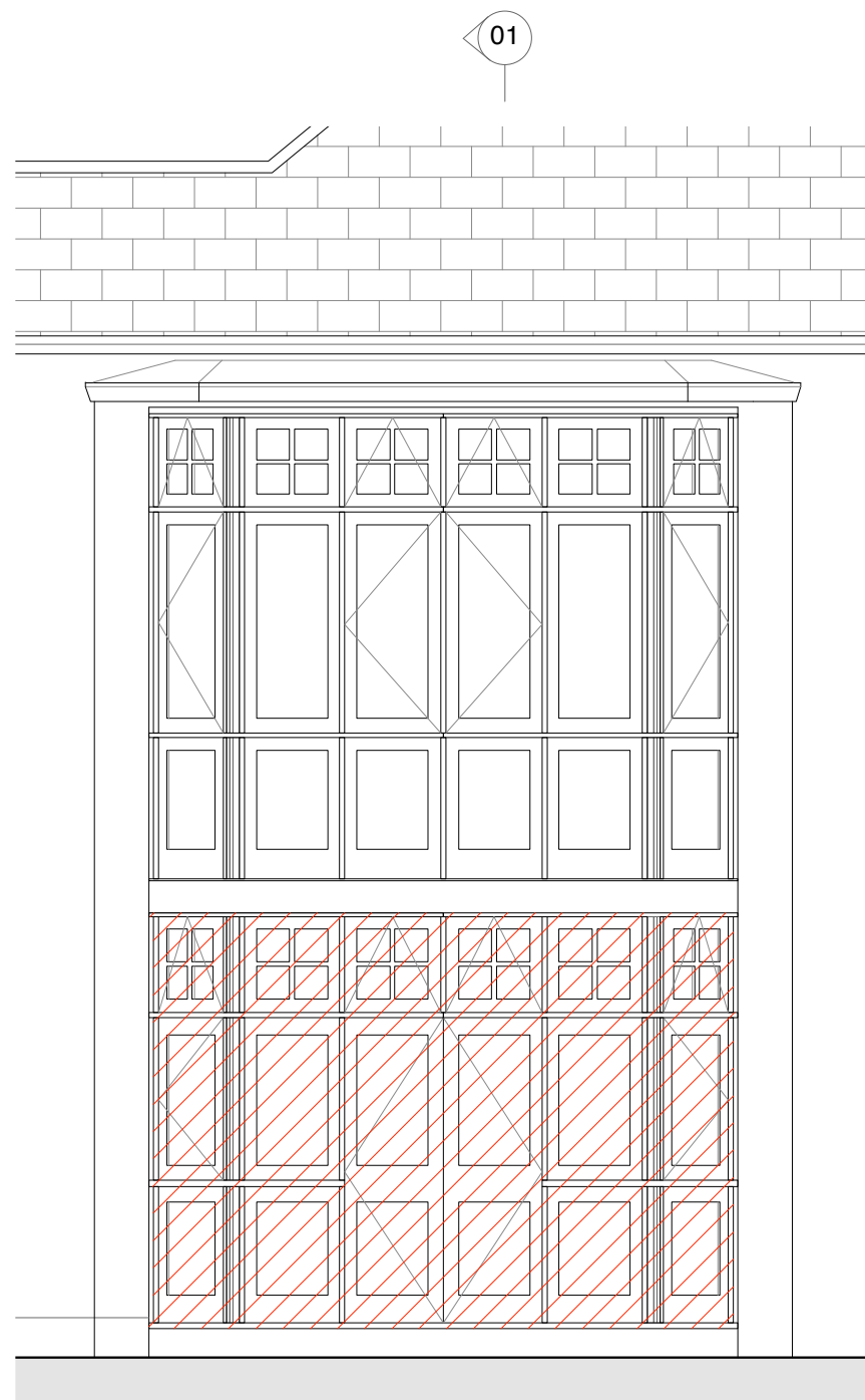
02 PL/14 Rear Elevation
