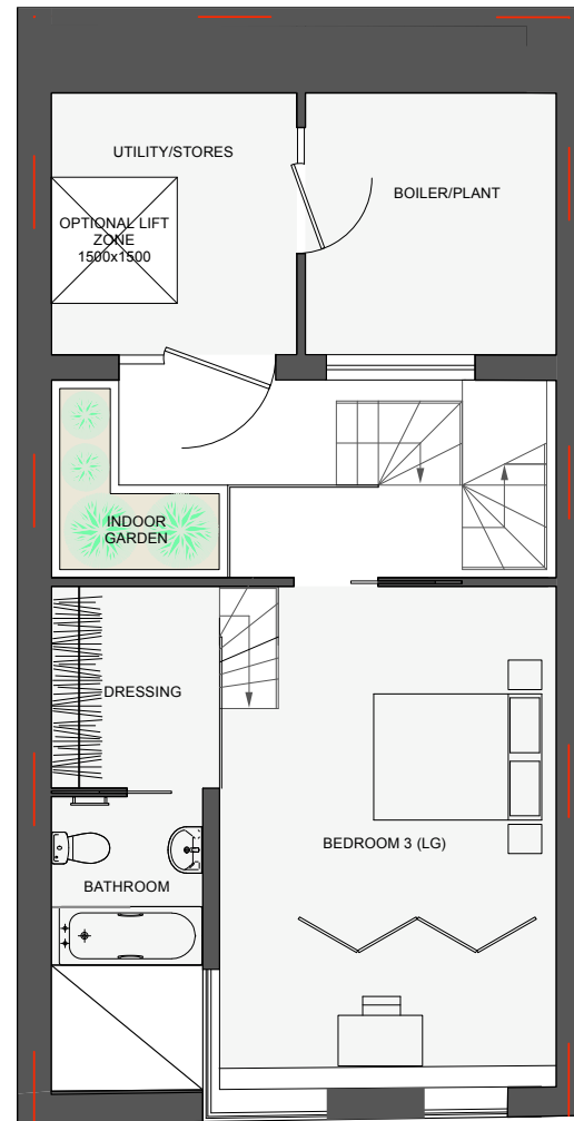
LOWER GROUND FLOOR PLAN LIFETIME HOME LAYOUT
