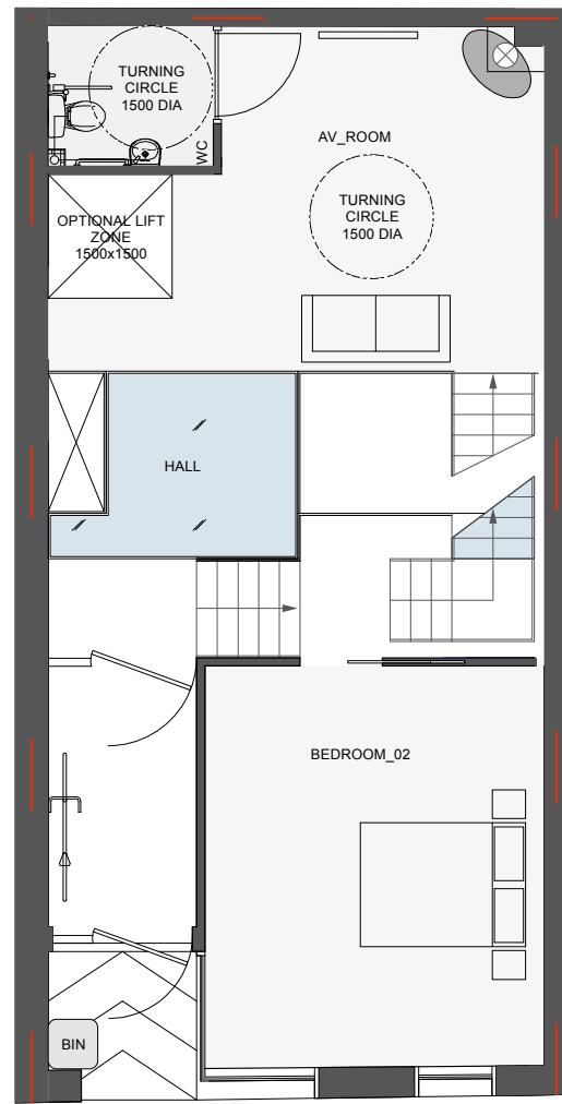
GROUND FLOOR PLAN LIFETIME HOME LAYOUT
