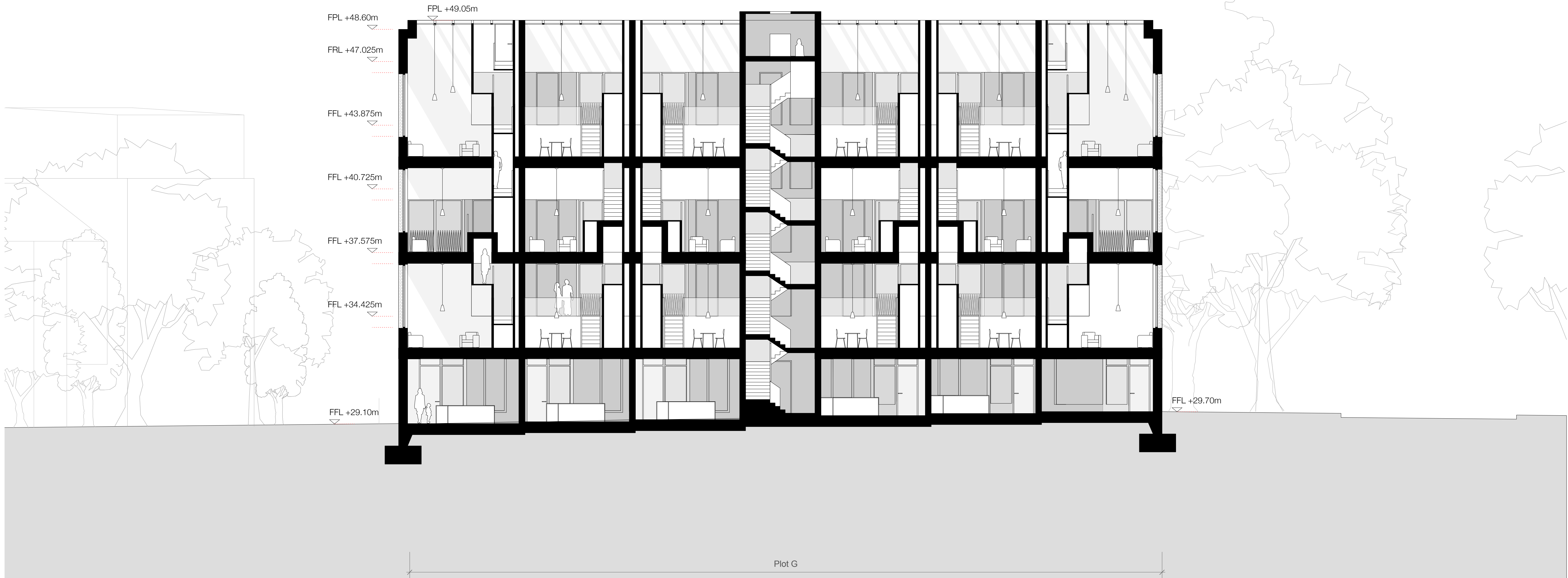
01 Section CC
