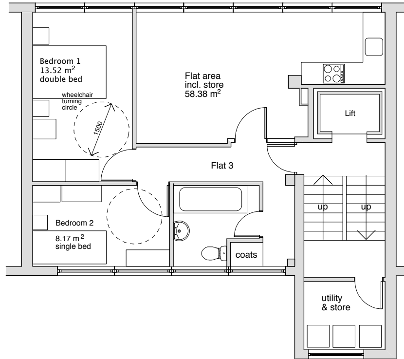
3rd Floor Plan
