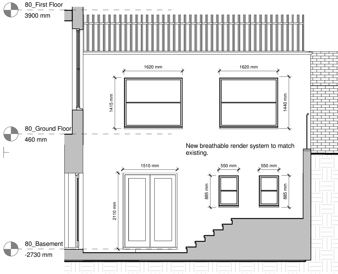
1:50 Proposed East Facing Elevation of Rear Extension
