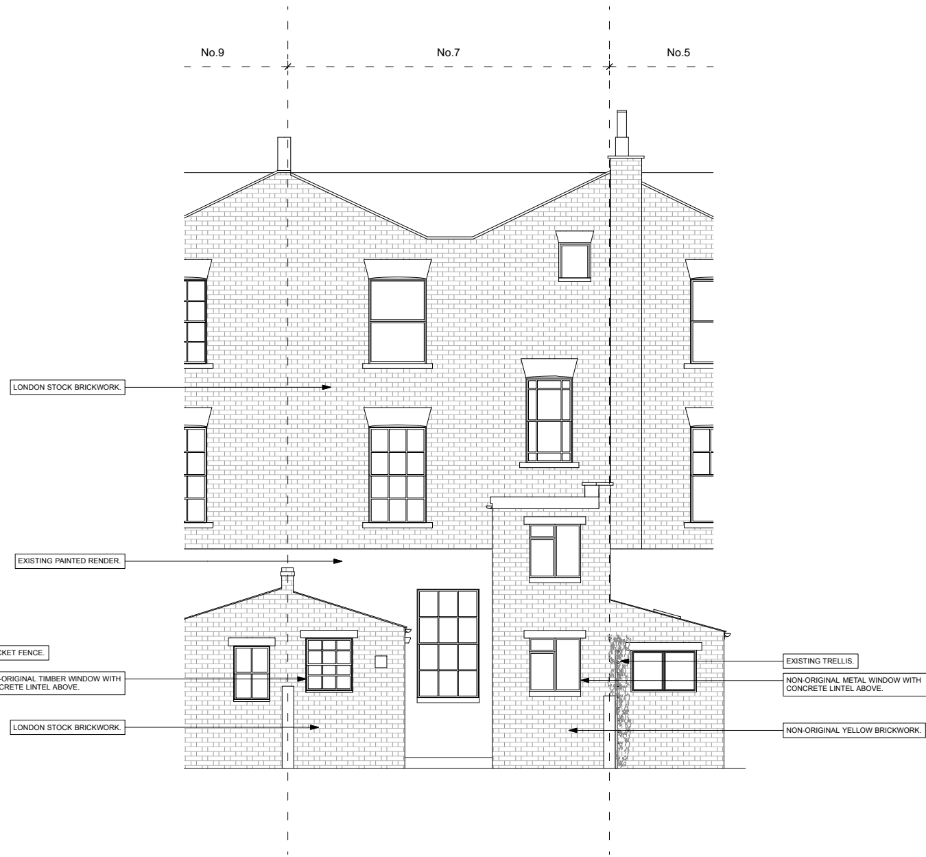
REAR ELEVATION
