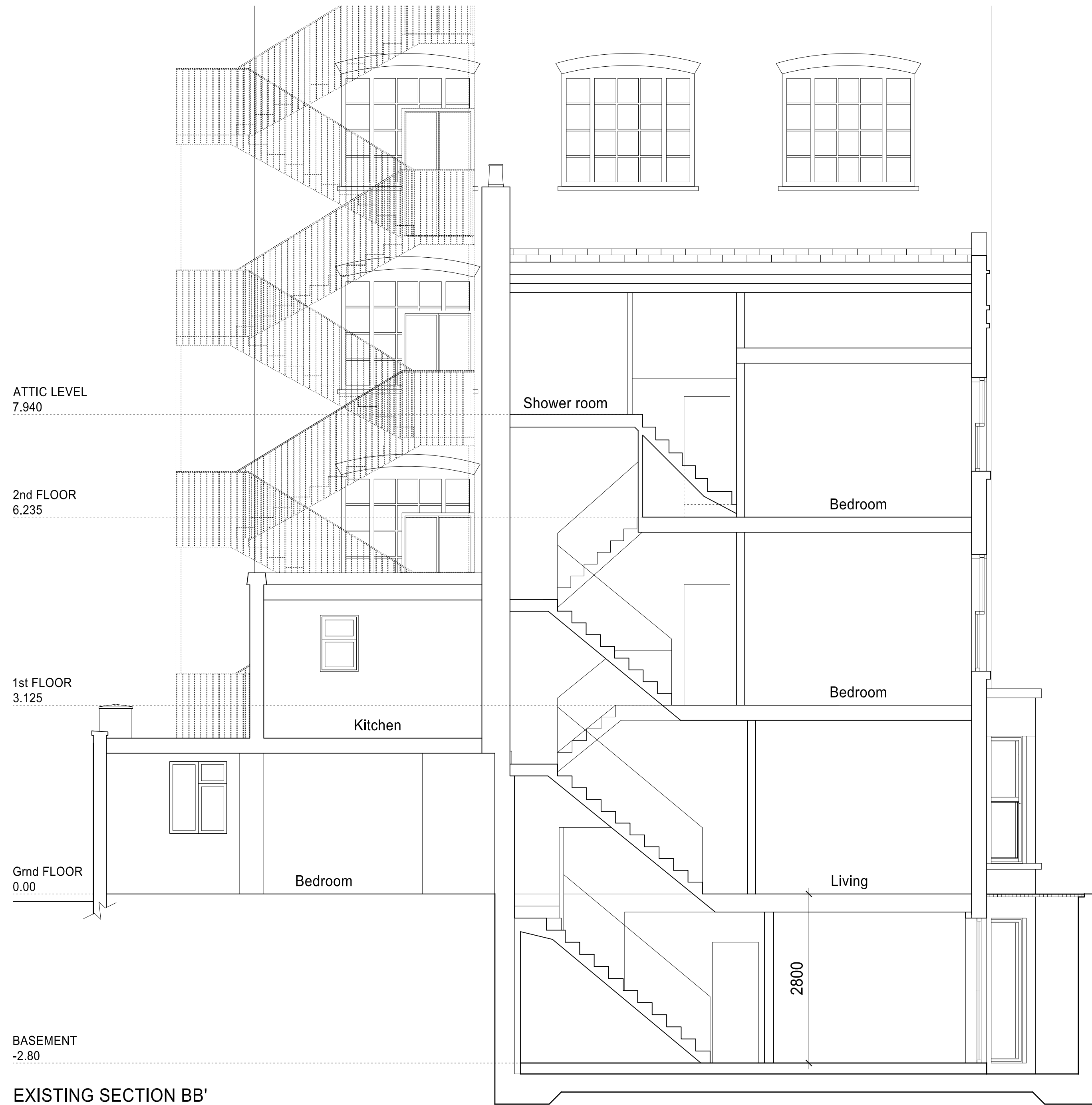
EXISTING SECTION BB' 10 BELMONT STREET
