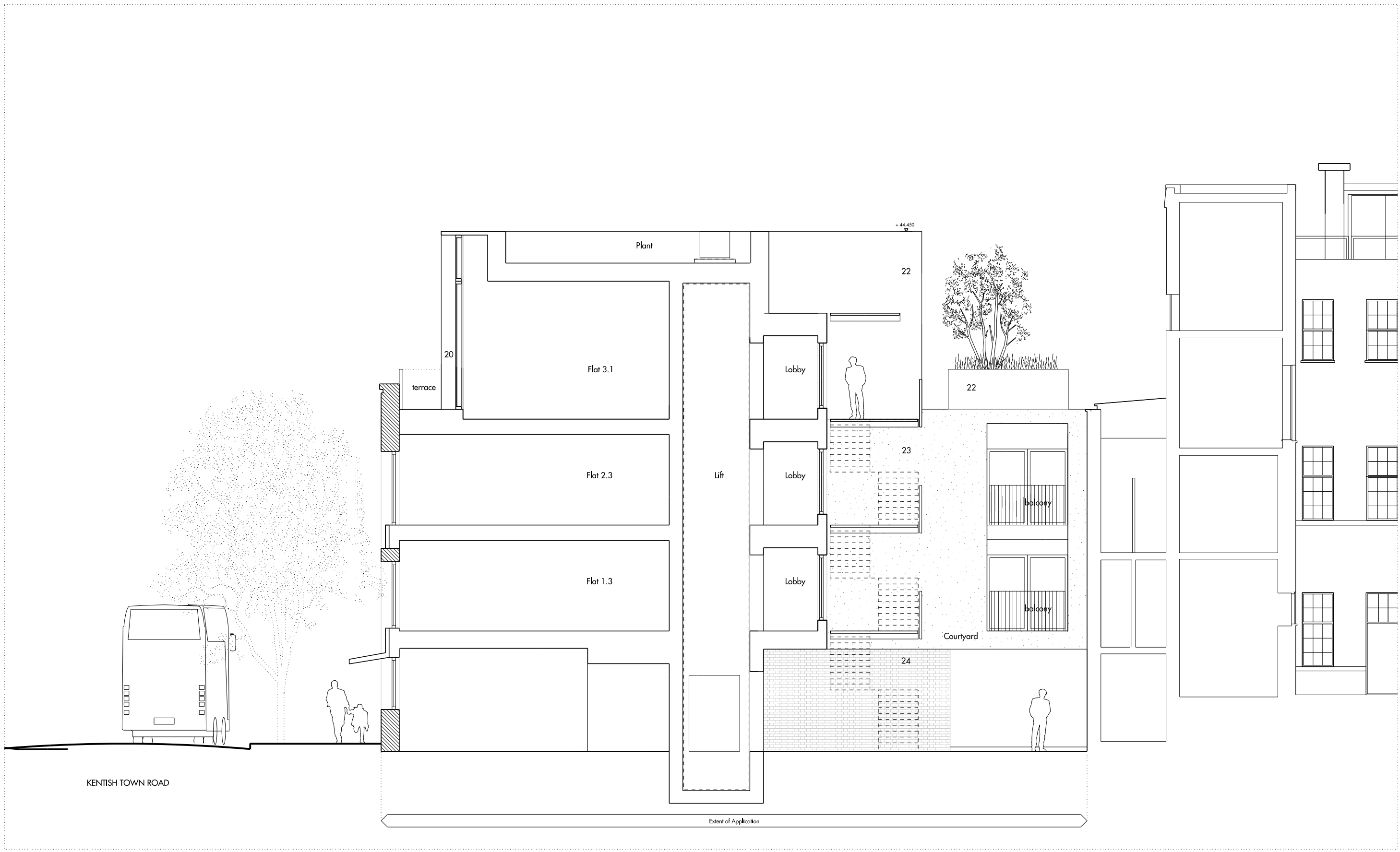
01 SECTION C - C (SOUTH) SCALE 1:50 @ A1
