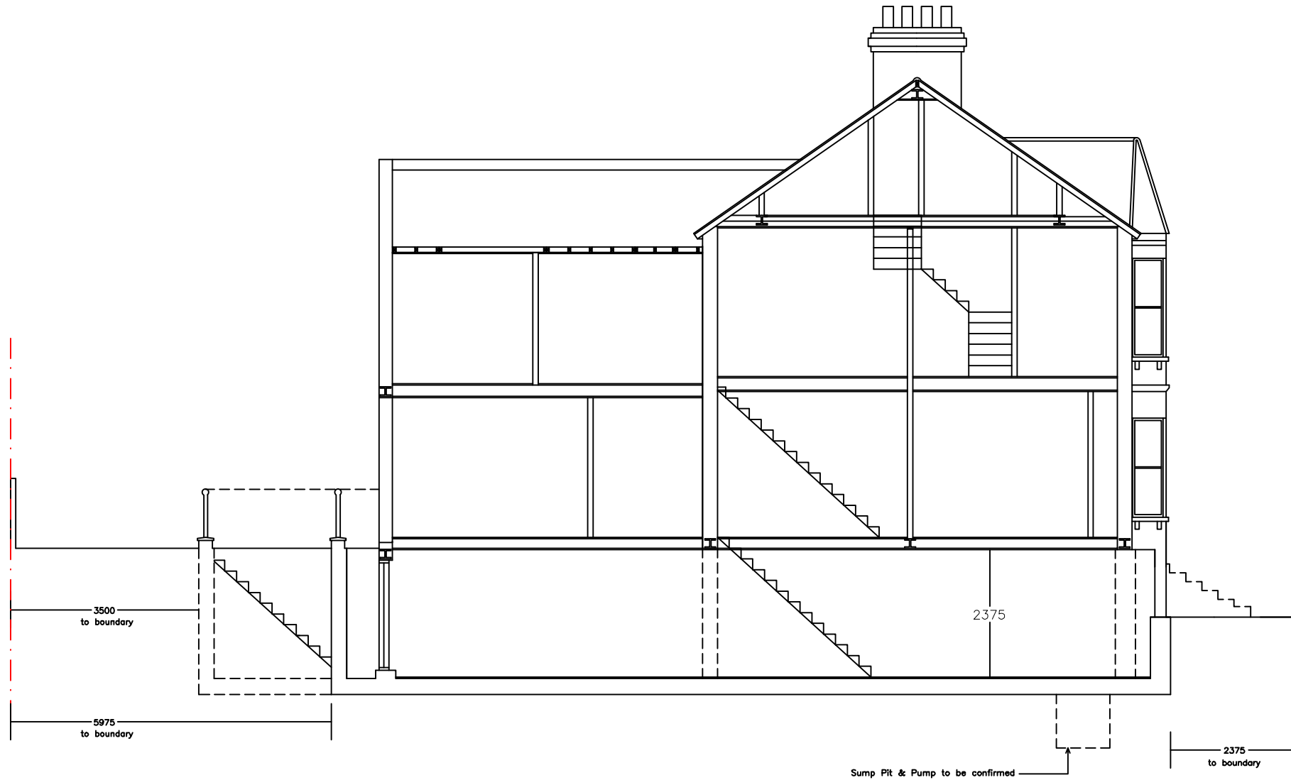
Proposed Section
