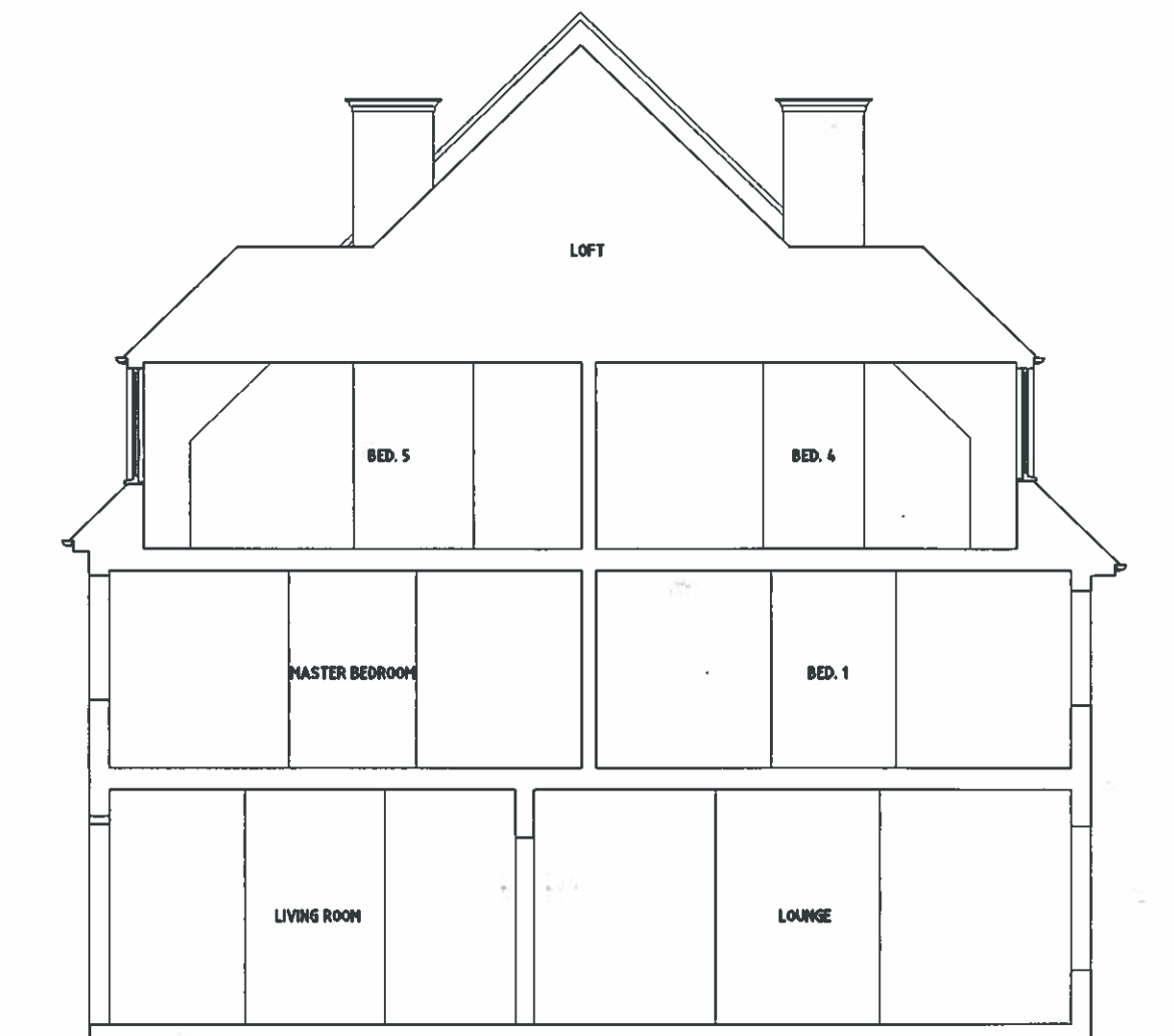
EXISTING SECTION
