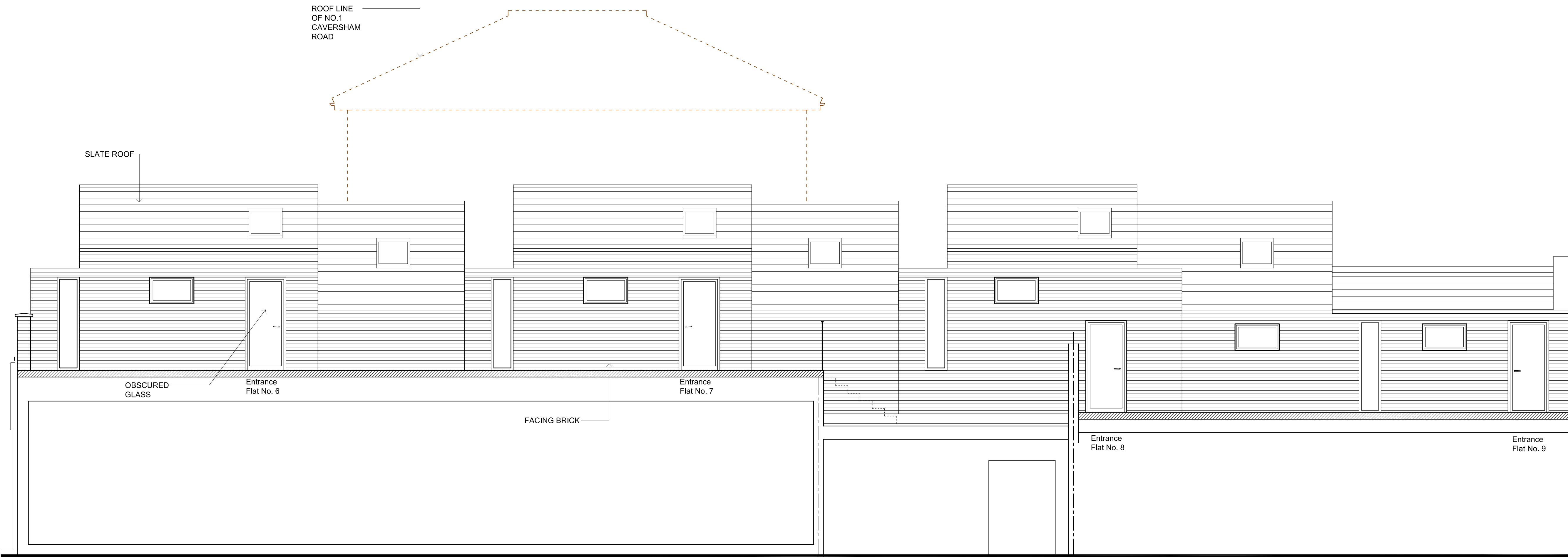
PROPOSED COURTYARD ELEVATION - PROPOSED MEWS
