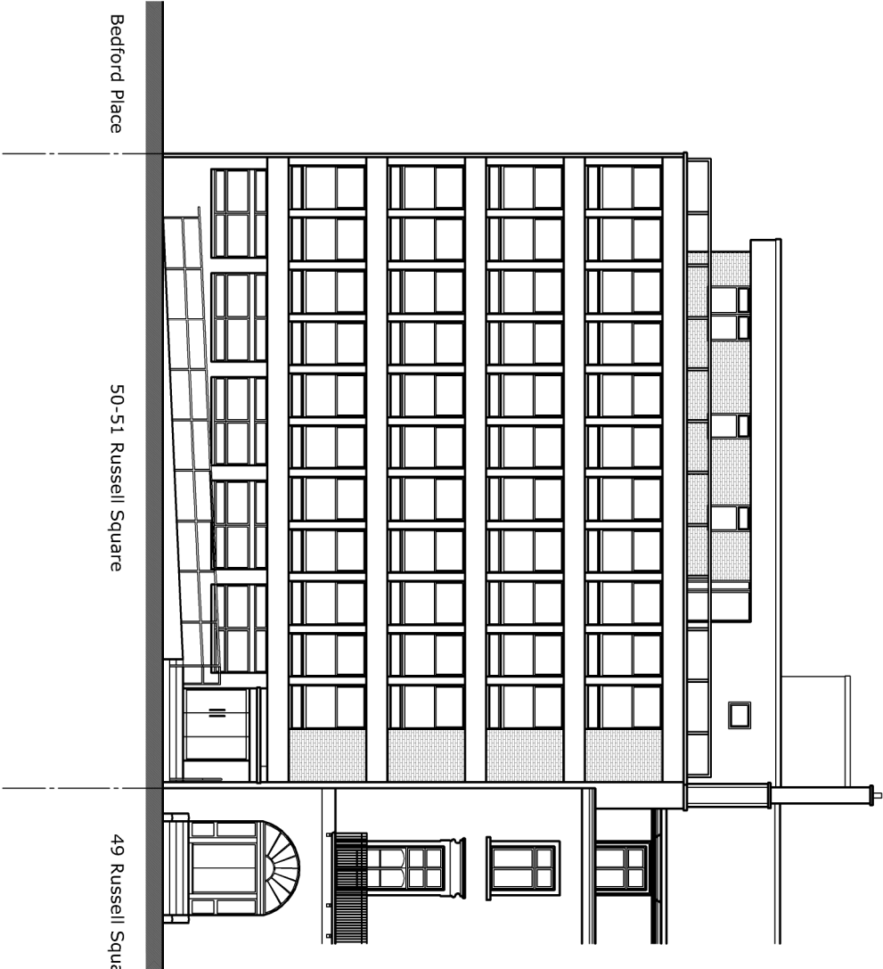
NORTH-EAST (FRONT) ELEVATION SCALE: 1:200
