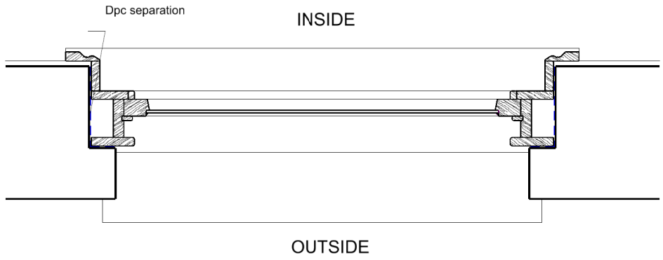
Plan Section Through Proposed 1-10
