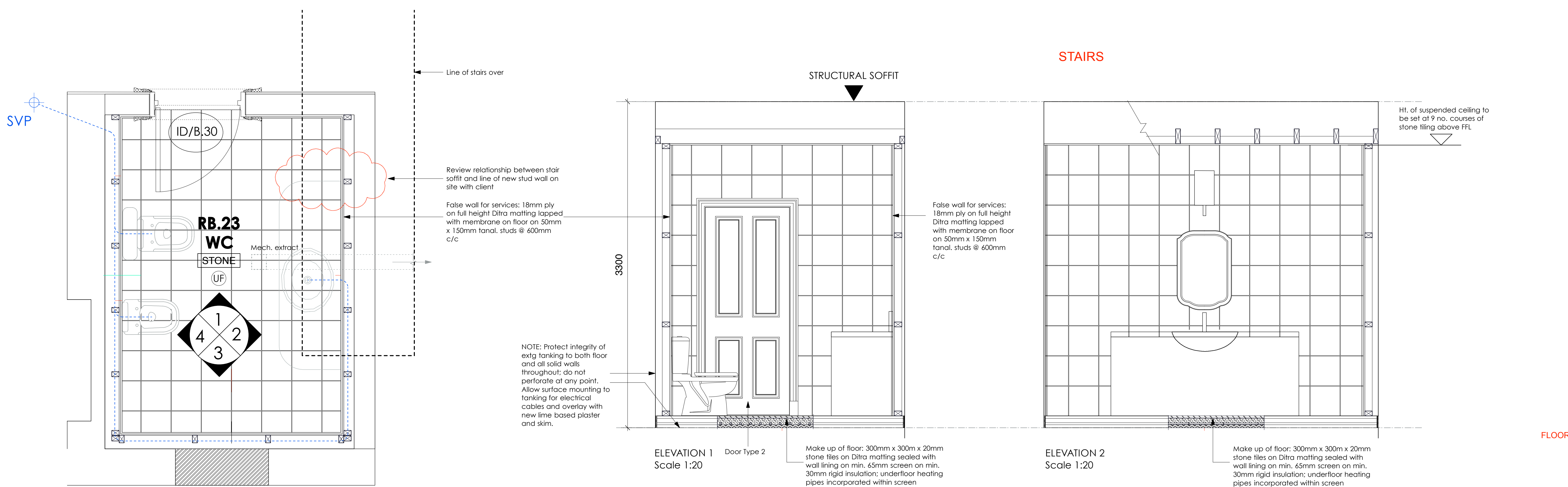
PLAN Scale 1:20
